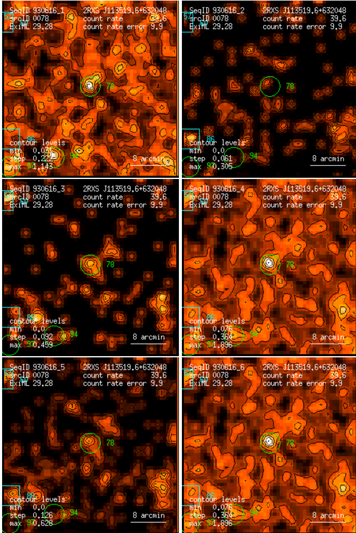
Figure 78: RASS 930616: detection 0078: band rate images, Gaussian filter: (1) PSPC channels 11 – 41, (2) 52 – 90, (3) 91 – 201, (4) 11 – 235, (5) 52 – 201, (6) 11 – 201. Broad band rates in counts/ks. Band rate contour levels in counts/ks/arcmin 2 .
