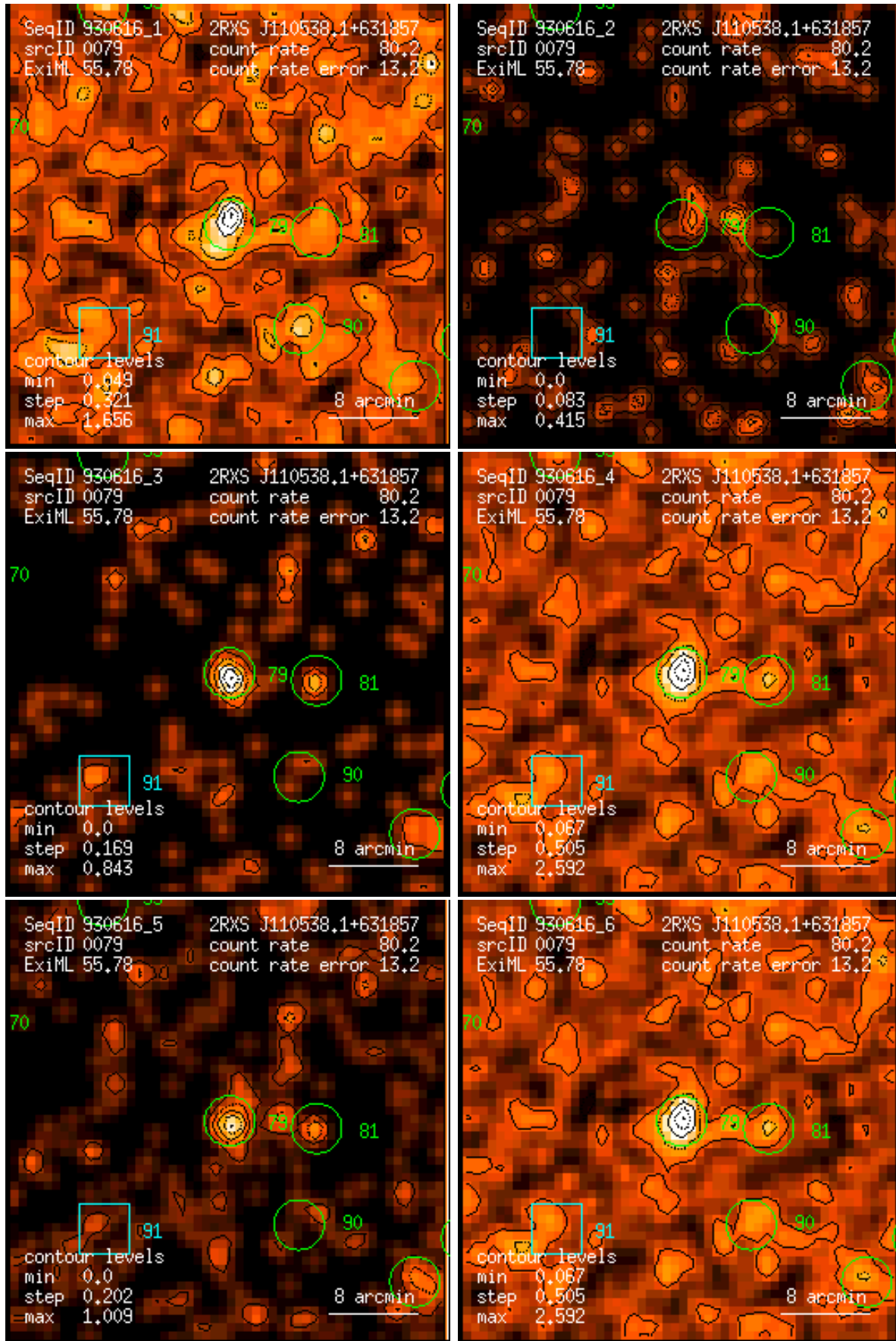
Figure 79: RASS 930616: detection 0079: band rate images, Gaussian filter: (1) PSPC channels 11 – 41, (2) 52 – 90, (3) 91 – 201, (4) 11 – 235, (5) 52 – 201, (6) 11 – 201. Broad band rates in counts/ks. Band rate contour levels in counts/ks/arcmin 2 .
