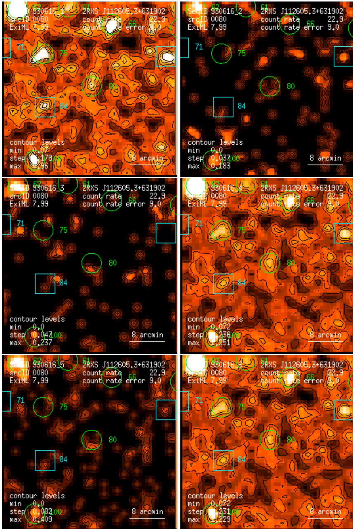
Figure 80: RASS 930616: detection 0080: band rate images, Gaussian filter: (1) PSPC channels 11 – 41, (2) 52 – 90, (3) 91 – 201, (4) 11 – 235, (5) 52 – 201, (6) 11 – 201. Broad band rates in counts/ks. Band rate contour levels in counts/ks/arcmin 2 .
