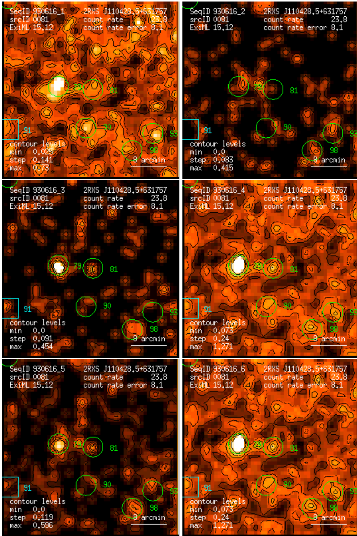
Figure 81: RASS 930616: detection 0081: band rate images, Gaussian filter: (1) PSPC channels 11 – 41, (2) 52 – 90, (3) 91 – 201, (4) 11 – 235, (5) 52 – 201, (6) 11 – 201. Broad band rates in counts/ks. Band rate contour levels in counts/ks/arcmin 2 .
