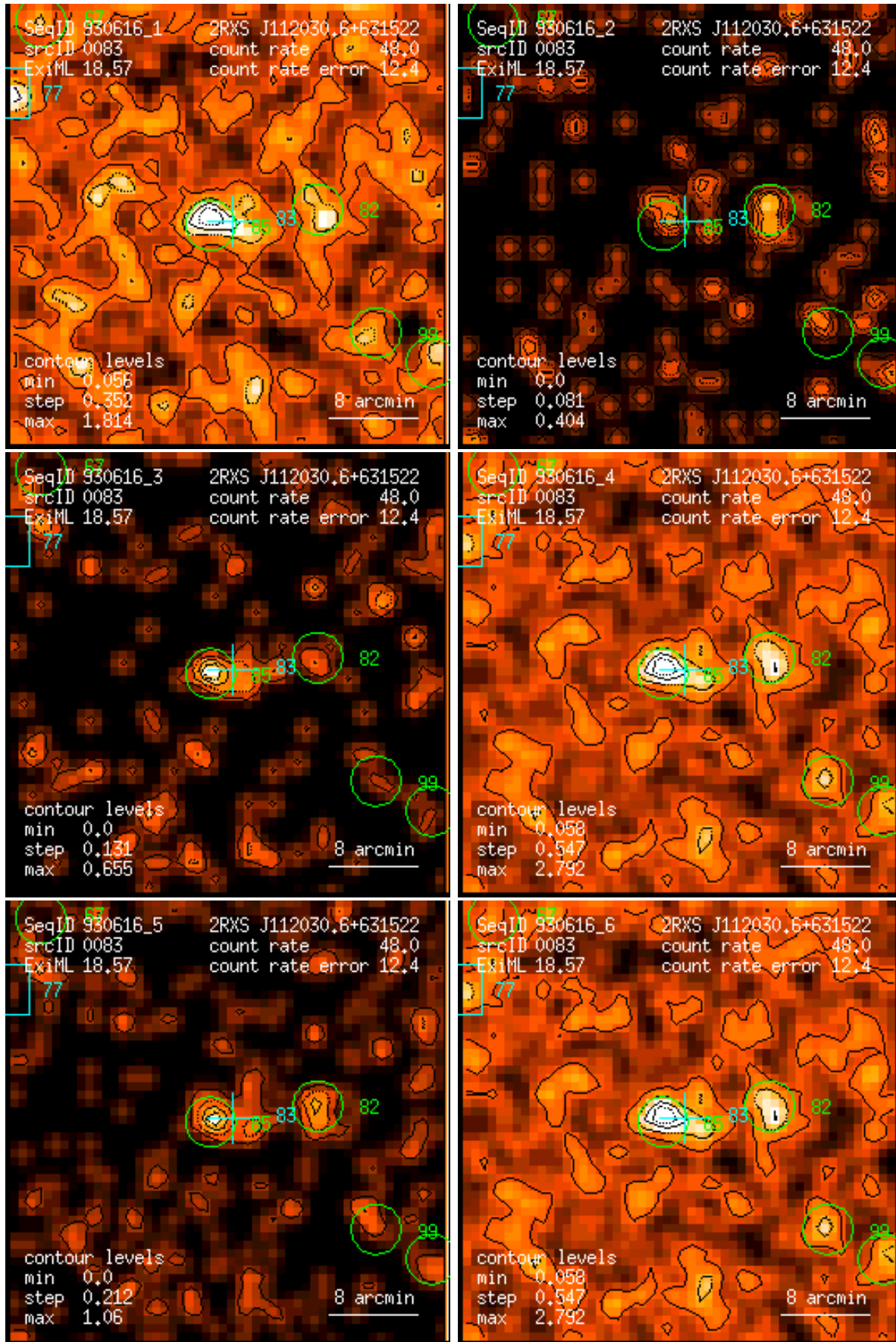
Figure 83: RASS 930616: detection 0083: band rate images, Gaussian filter: (1) PSPC channels 11 – 41, (2) 52 – 90, (3) 91 – 201, (4) 11 – 235, (5) 52 – 201, (6) 11 – 201. Broad band rates in counts/ks. Band rate contour levels in counts/ks/arcmin 2 .
