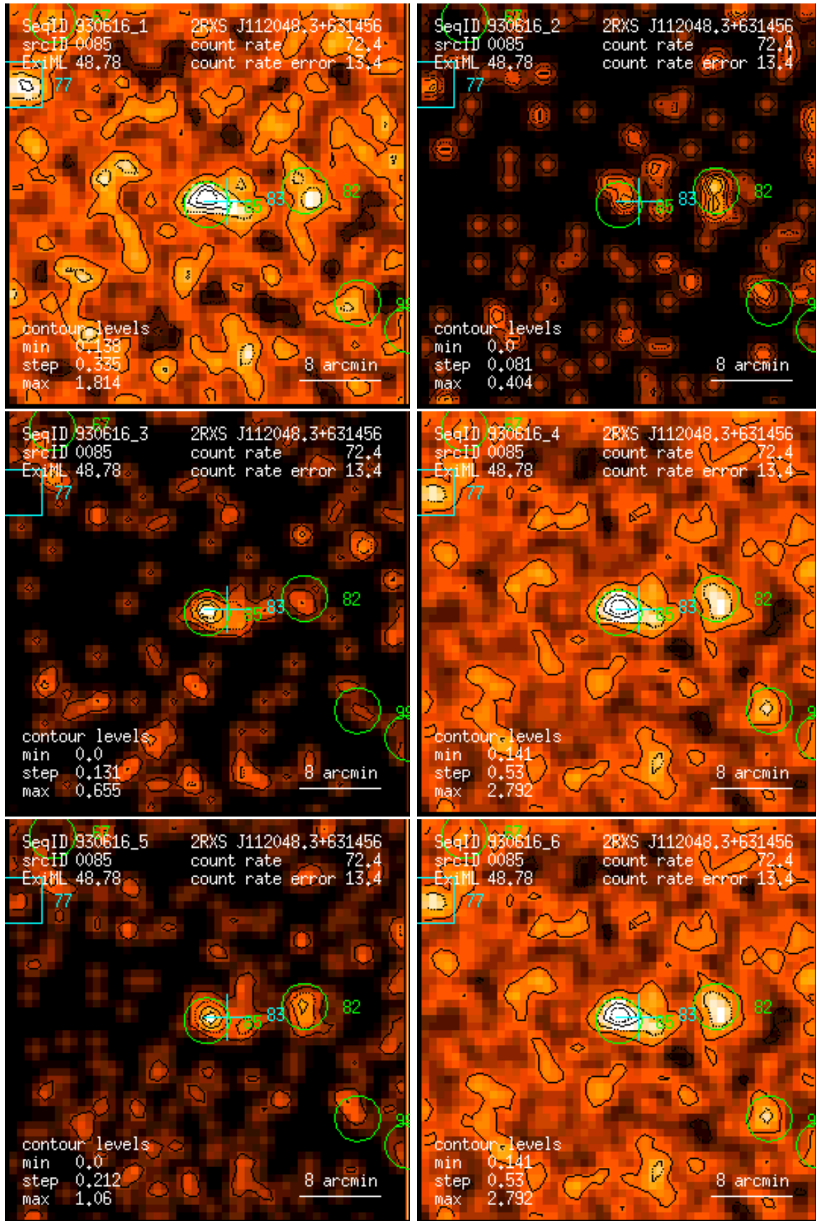
Figure 85: RASS 930616: detection 0085: band rate images, Gaussian filter: (1) PSPC channels 11 – 41, (2) 52 – 90, (3) 91 – 201, (4) 11 – 235, (5) 52 – 201, (6) 11 – 201. Broad band rates in counts/ks. Band rate contour levels in counts/ks/arcmin 2 .
