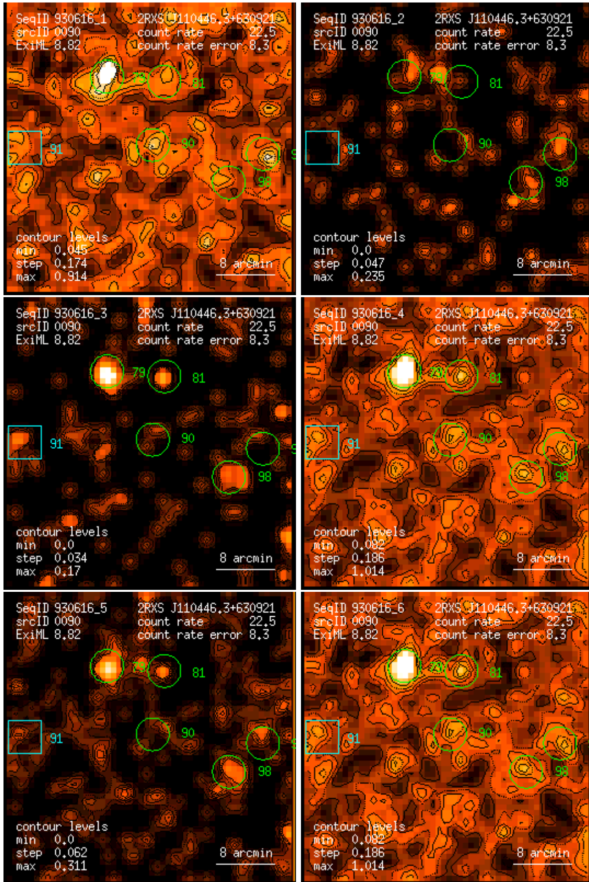
Figure 90: RASS 930616: detection 0090: band rate images, Gaussian filter: (1) PSPC channels 11 – 41, (2) 52 – 90, (3) 91 – 201, (4) 11 – 235, (5) 52 – 201, (6) 11 – 201. Broad band rates in counts/ks. Band rate contour levels in counts/ks/arcmin 2 .
