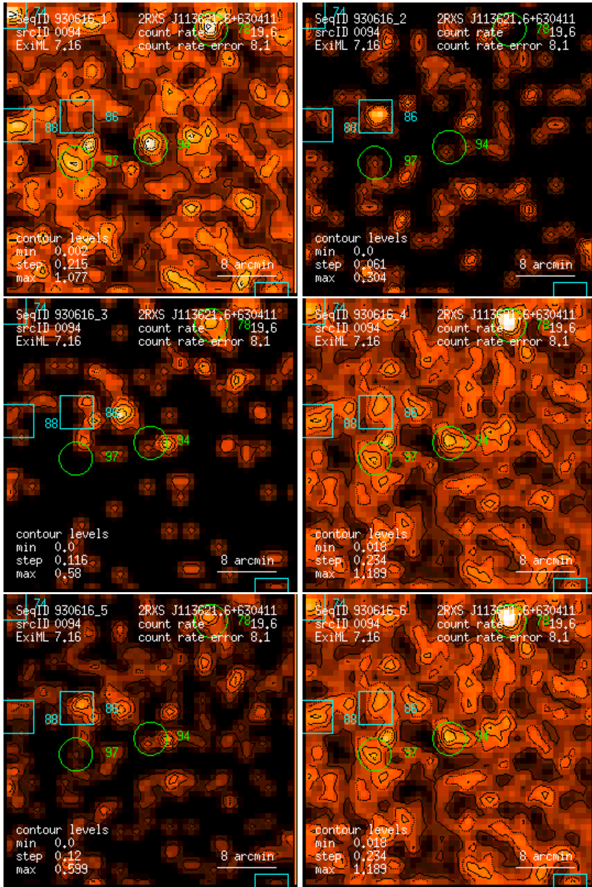
Figure 94: RASS 930616: detection 0094: band rate images, Gaussian filter: (1) PSPC channels 11 – 41, (2) 52 – 90, (3) 91 – 201, (4) 11 – 235, (5) 52 – 201, (6) 11 – 201. Broad band rates in counts/ks. Band rate contour levels in counts/ks/arcmin 2 .
