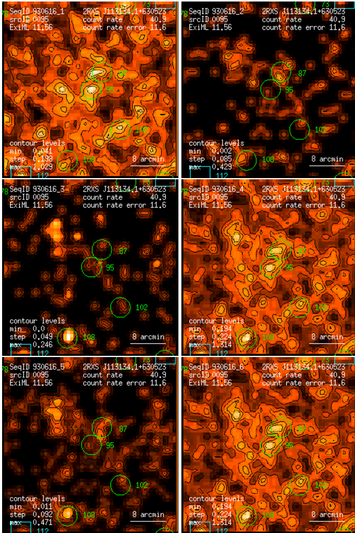
Figure 95: RASS 930616: detection 0095: band rate images, Gaussian filter: (1) PSPC channels 11 – 41, (2) 52 – 90, (3) 91 – 201, (4) 11 – 235, (5) 52 – 201, (6) 11 – 201. Broad band rates in counts/ks. Band rate contour levels in counts/ks/arcmin 2 .
