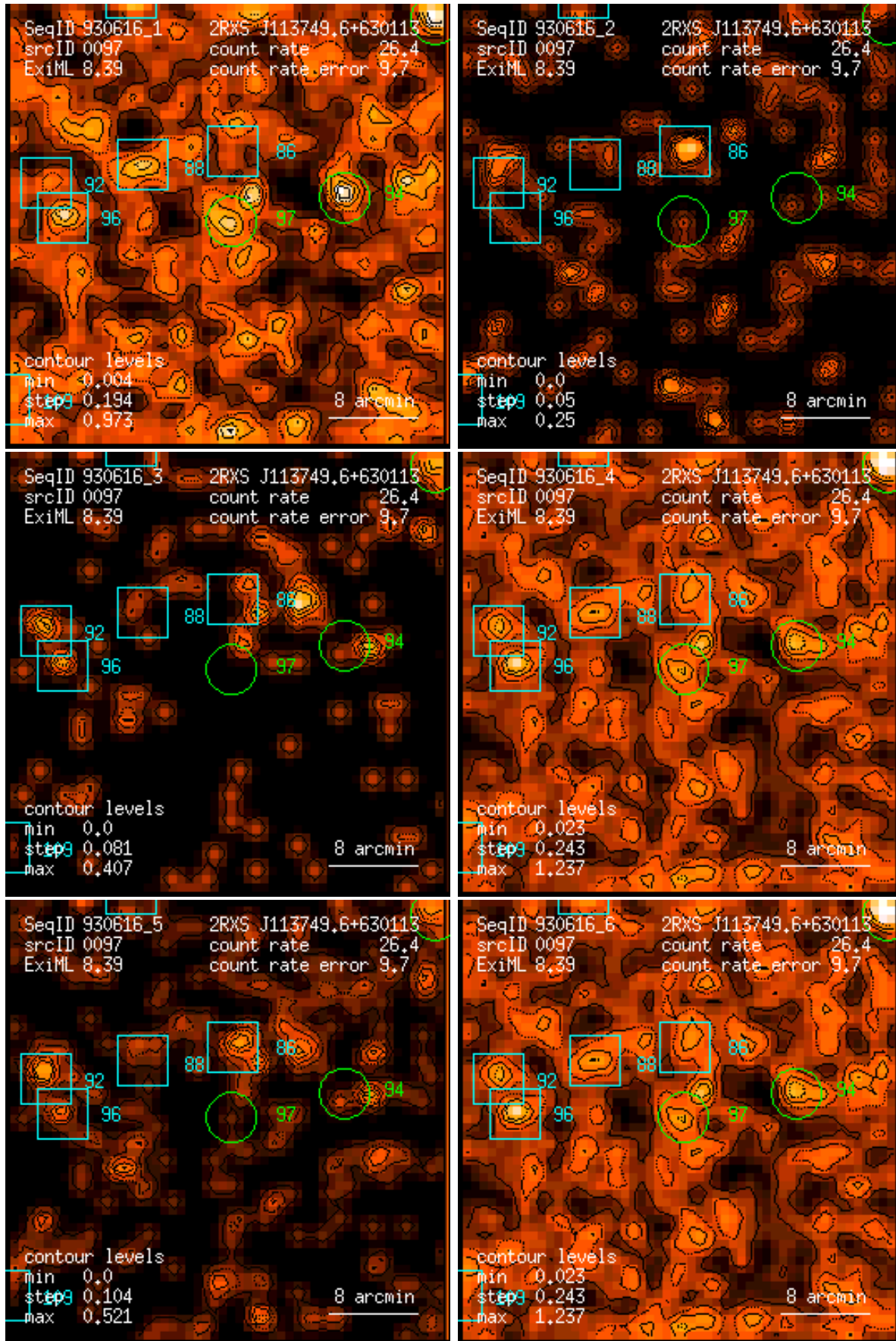
Figure 97: RASS 930616: detection 0097: band rate images, Gaussian filter: (1) PSPC channels 11 – 41, (2) 52 – 90, (3) 91 – 201, (4) 11 – 235, (5) 52 – 201, (6) 11 – 201. Broad band rates in counts/ks. Band rate contour levels in counts/ks/arcmin 2 .
