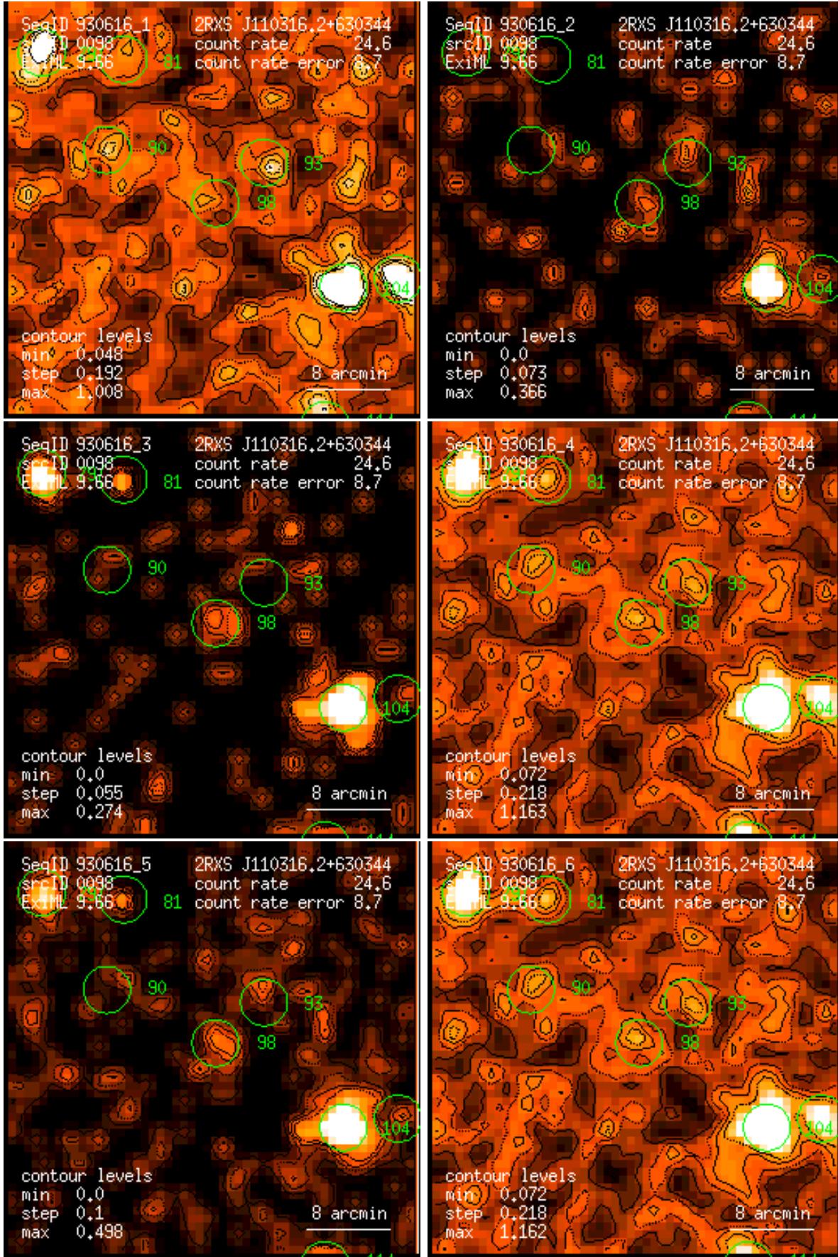
Figure 98: RASS 930616: detection 0098: band rate images, Gaussian filter: (1) PSPC channels 11 – 41, (2) 52 – 90, (3) 91 – 201, (4) 11 – 235, (5) 52 – 201, (6) 11 – 201. Broad band rates in counts/ks. Band rate contour levels in counts/ks/arcmin 2 .
