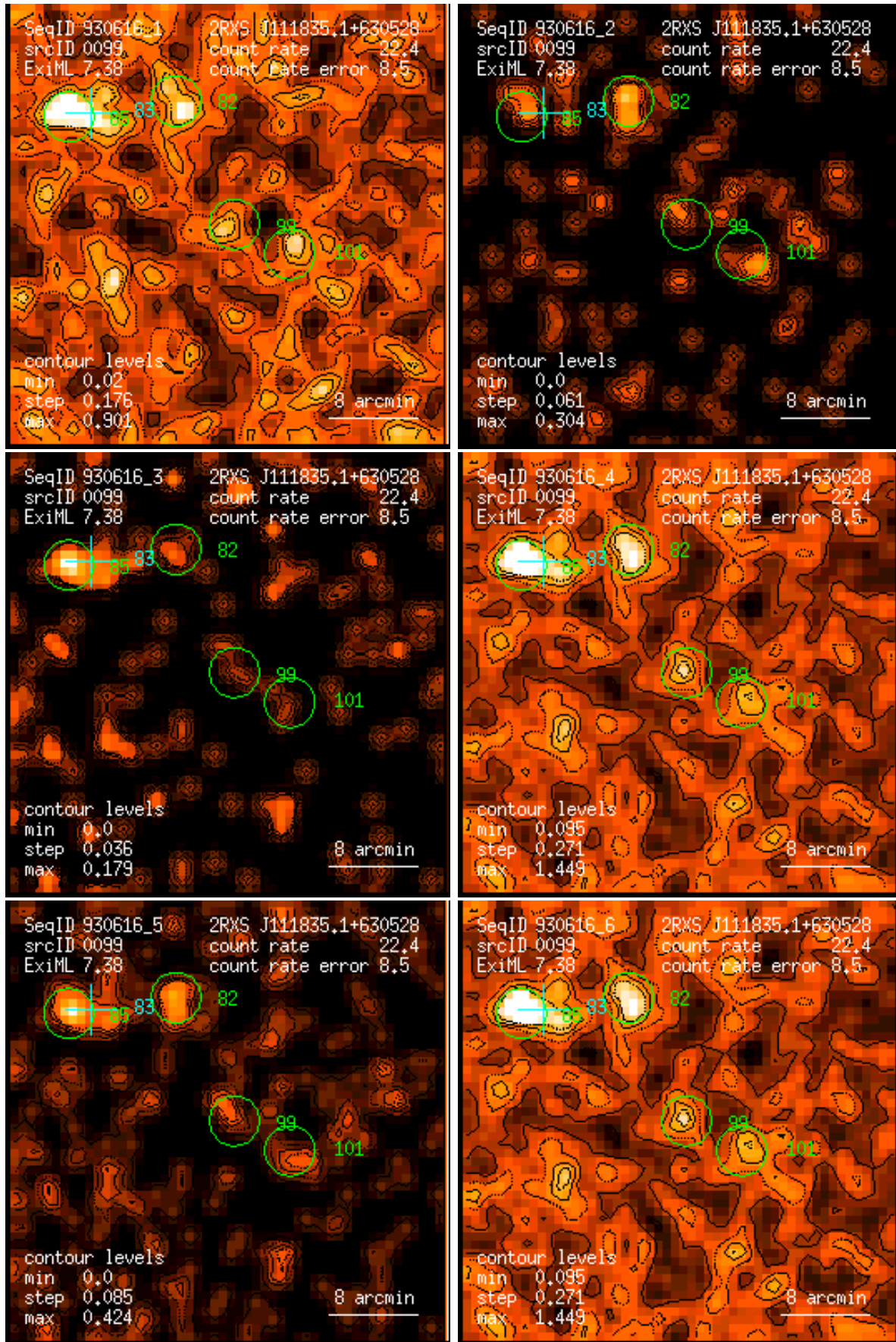
Figure 99: RASS 930616: detection 0099: band rate images, Gaussian filter: (1) PSPC channels 11 – 41, (2) 52 – 90, (3) 91 – 201, (4) 11 – 235, (5) 52 – 201, (6) 11 – 201. Broad band rates in counts/ks. Band rate contour levels in counts/ks/arcmin 2 .
