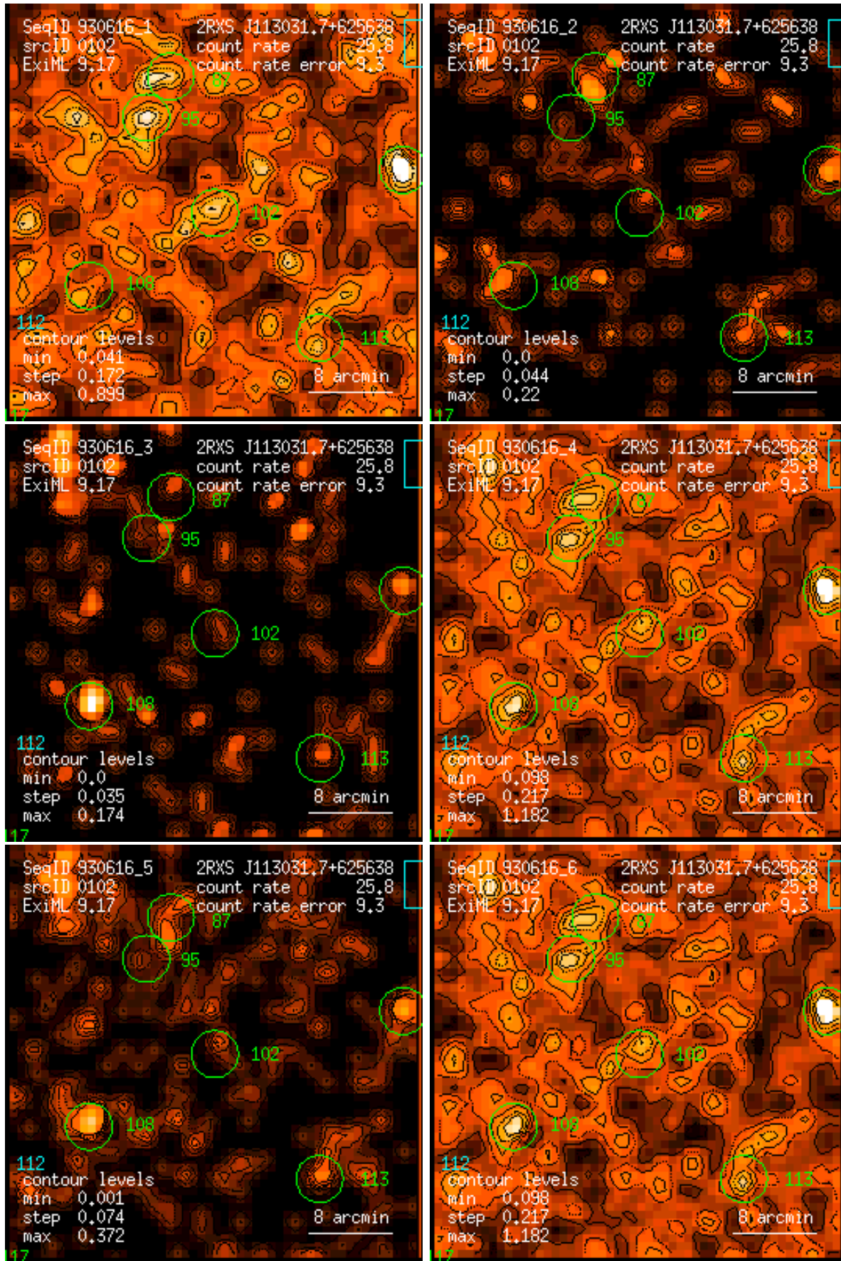
Figure 102: RASS 930616: detection 0102: band rate images, Gaussian filter: (1) PSPC channels 11 – 41, (2) 52 – 90, (3) 91 – 201, (4) 11 – 235, (5) 52 – 201, (6) 11 – 201. Broad band rates in counts/ks. Band rate contour levels in counts/ks/arcmin 2 .
