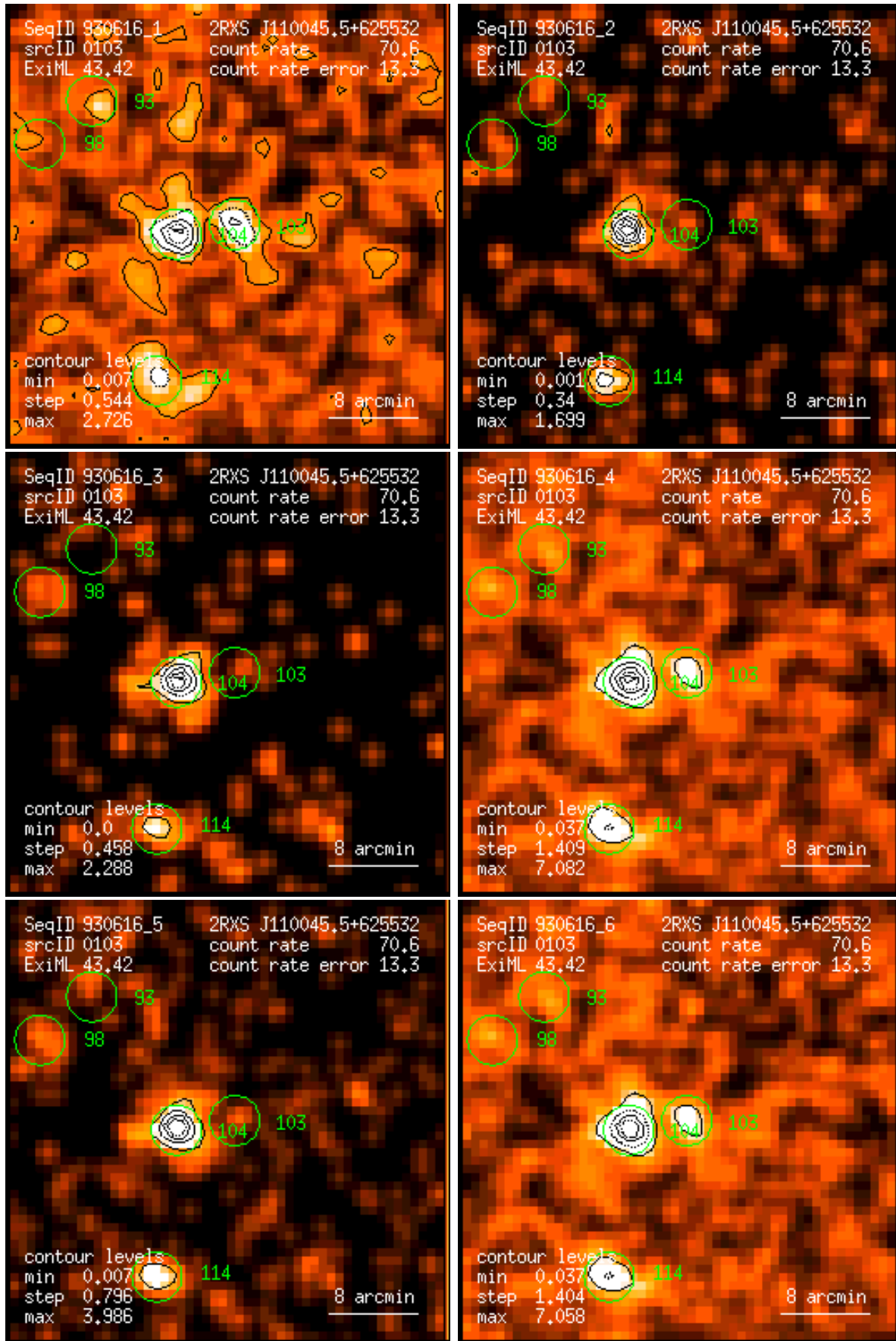
Figure 103: RASS 930616: detection 0103: band rate images, Gaussian filter: (1) PSPC channels 11 – 41, (2) 52 – 90, (3) 91 – 201, (4) 11 – 235, (5) 52 – 201, (6) 11 – 201. Broad band rates in counts/ks. Band rate contour levels in counts/ks/arcmin 2 .
