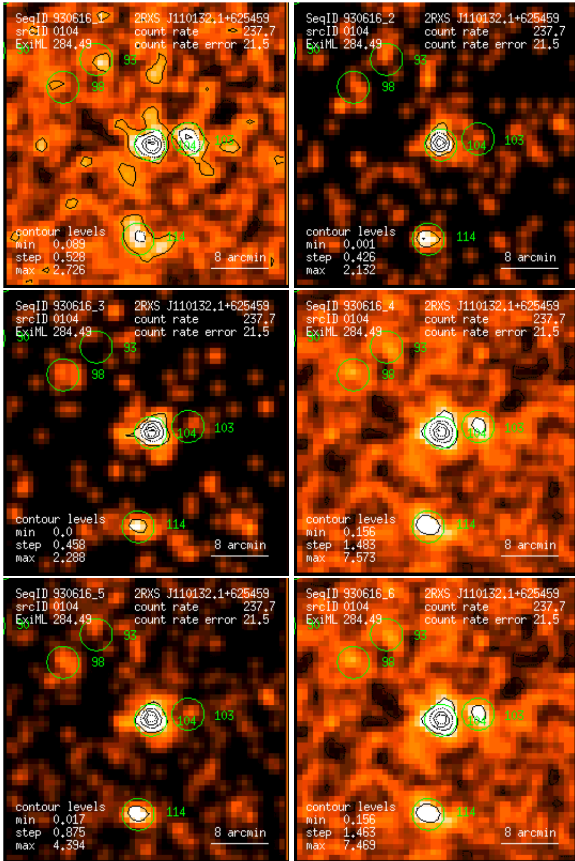
Figure 104: RASS 930616: detection 0104: band rate images, Gaussian filter: (1) PSPC channels 11 – 41, (2) 52 – 90, (3) 91 – 201, (4) 11 – 235, (5) 52 – 201, (6) 11 – 201. Broad band rates in counts/ks. Band rate contour levels in counts/ks/arcmin 2 .
