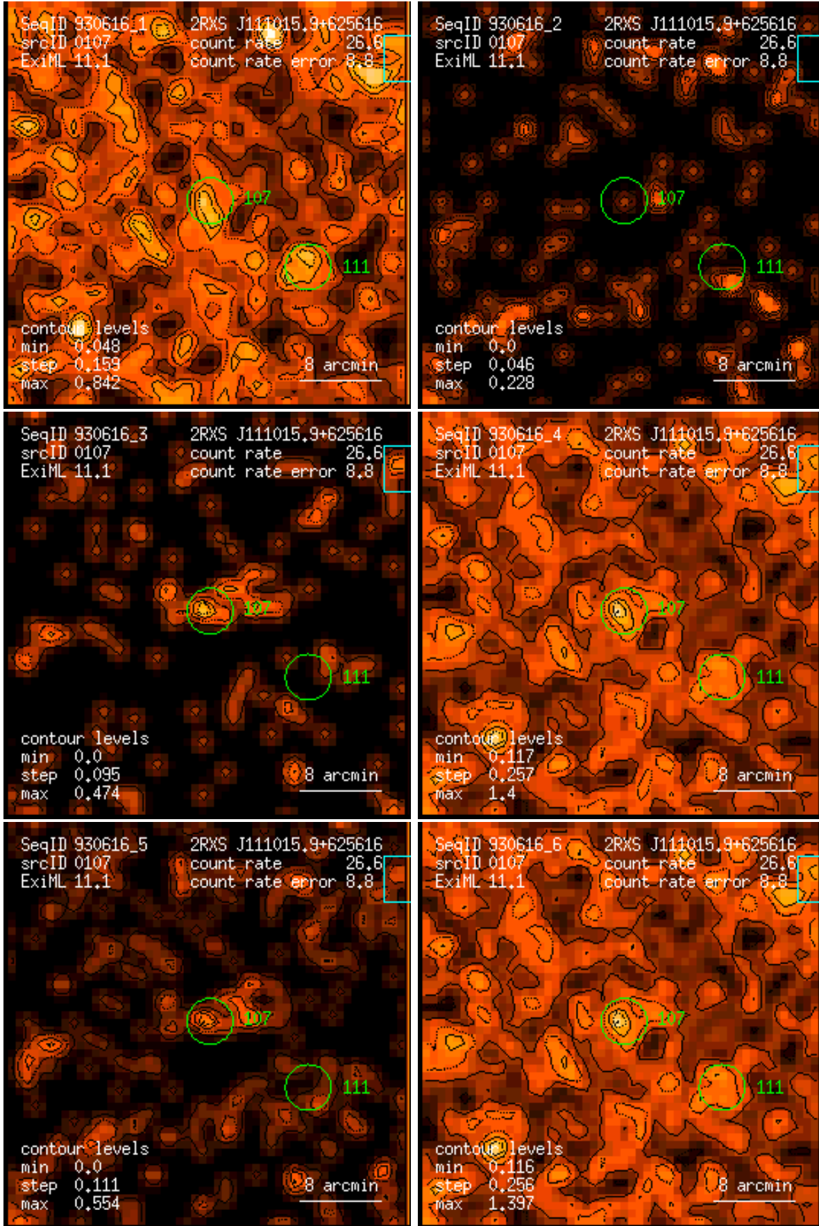
Figure 107: RASS 930616: detection 0107: band rate images, Gaussian filter: (1) PSPC channels 11 – 41, (2) 52 – 90, (3) 91 – 201, (4) 11 – 235, (5) 52 – 201, (6) 11 – 201. Broad band rates in counts/ks. Band rate contour levels in counts/ks/arcmin 2 .
