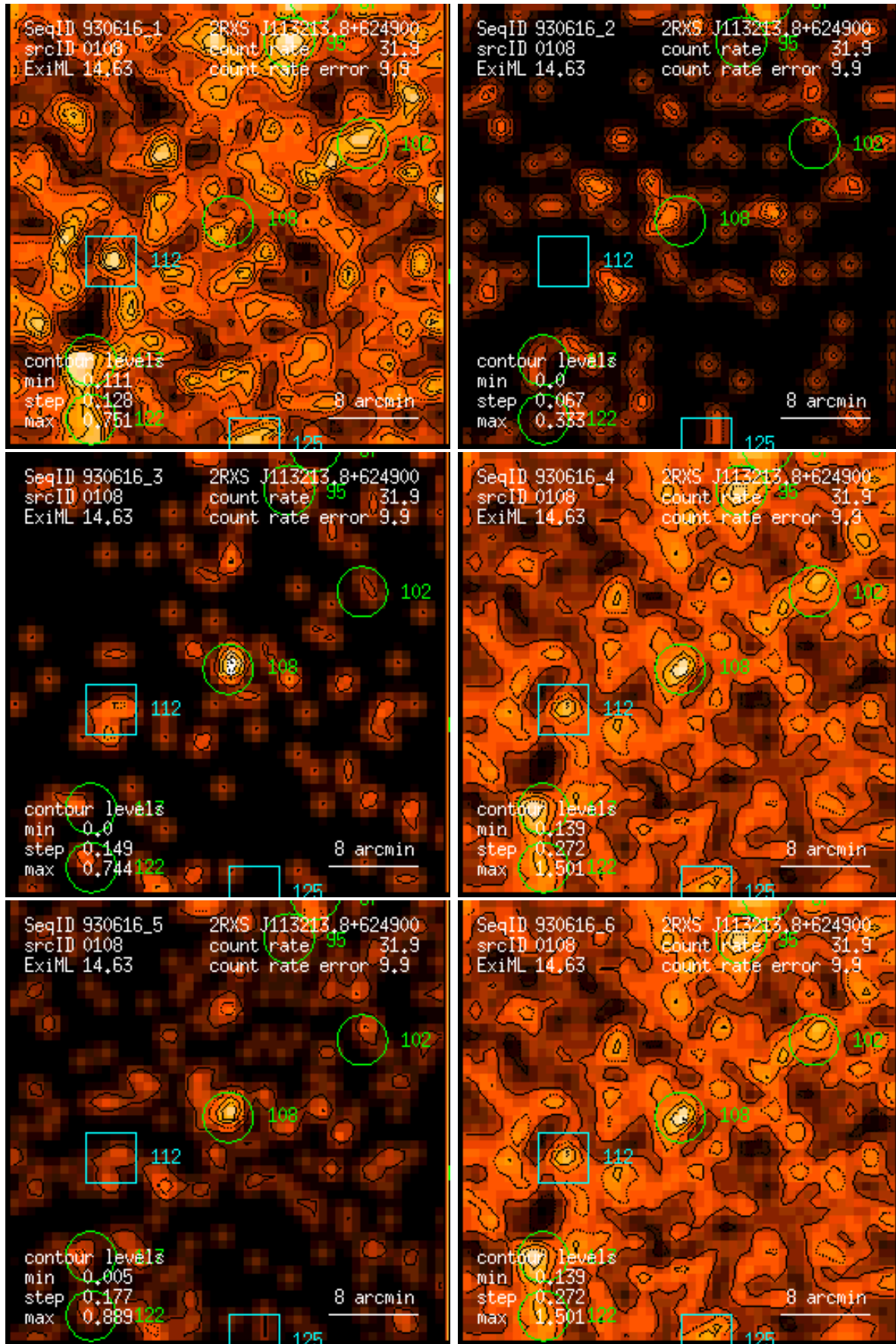
Figure 108: RASS 930616: detection 0108: band rate images, Gaussian filter: (1) PSPC channels 11 – 41, (2) 52 – 90, (3) 91 – 201, (4) 11 – 235, (5) 52 – 201, (6) 11 – 201. Broad band rates in counts/ks. Band rate contour levels in counts/ks/arcmin 2 .
