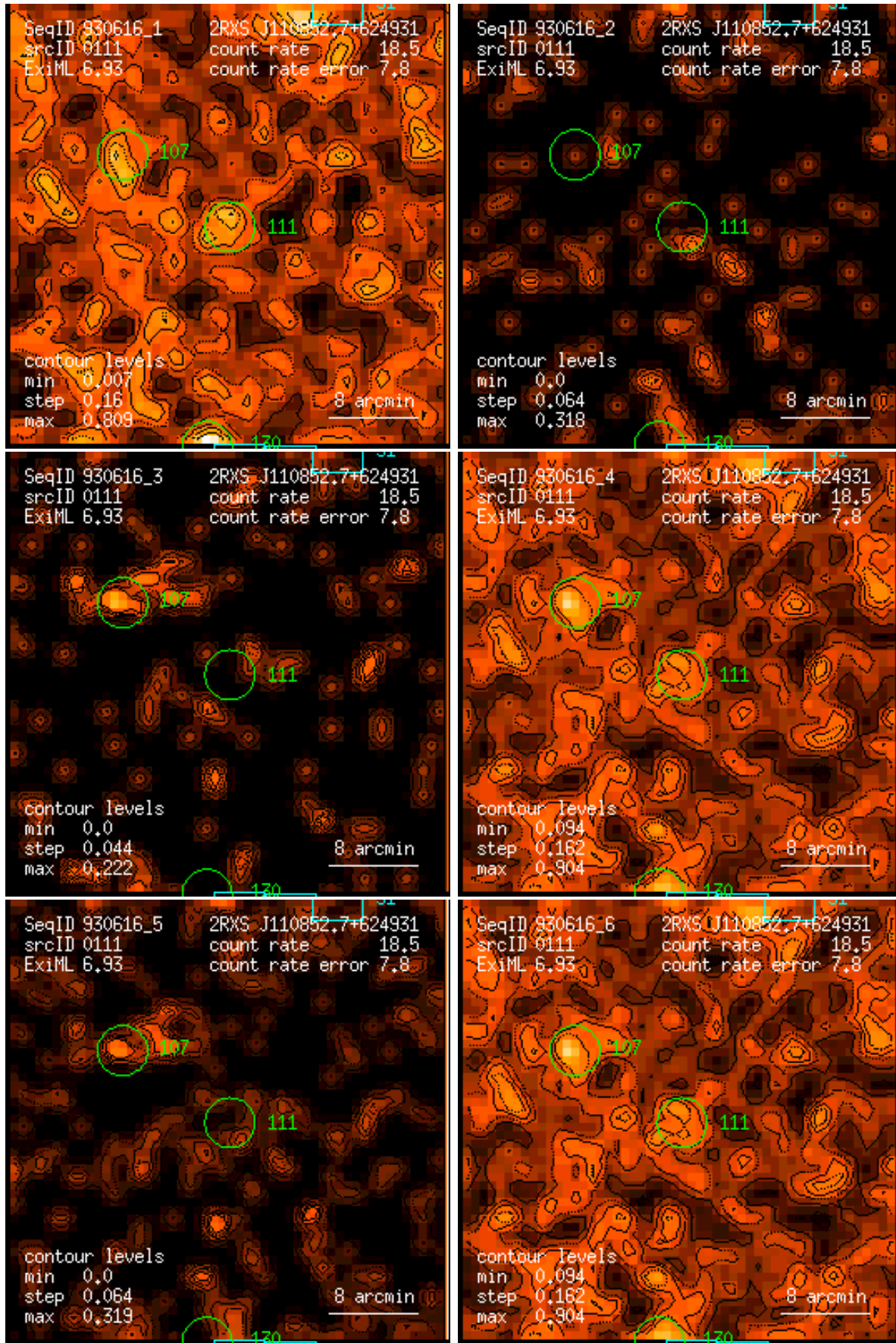
Figure 111: RASS 930616: detection 0111: band rate images, Gaussian filter: (1) PSPC channels 11 – 41, (2) 52 – 90, (3) 91 – 201, (4) 11 – 235, (5) 52 – 201, (6) 11 – 201. Broad band rates in counts/ks. Band rate contour levels in counts/ks/arcmin 2 .
