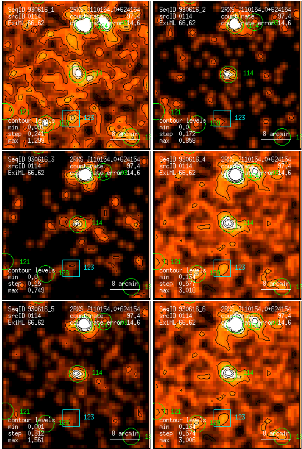
Figure 114: RASS 930616: detection 0114: band rate images, Gaussian filter: (1) PSPC channels 11 – 41, (2) 52 – 90, (3) 91 – 201, (4) 11 – 235, (5) 52 – 201, (6) 11 – 201. Broad band rates in counts/ks. Band rate contour levels in counts/ks/arcmin 2 .
