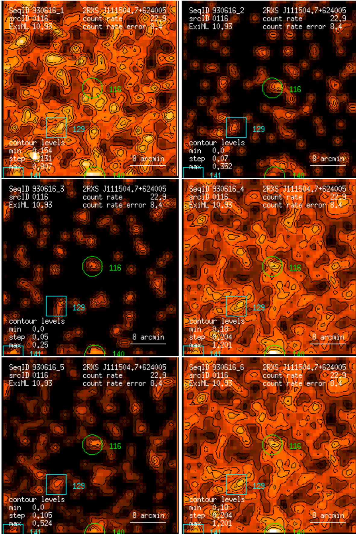
Figure 116: RASS 930616: detection 0116: band rate images, Gaussian filter: (1) PSPC channels 11 – 41, (2) 52 – 90, (3) 91 – 201, (4) 11 – 235, (5) 52 – 201, (6) 11 – 201. Broad band rates in counts/ks. Band rate contour levels in counts/ks/arcmin 2 .
