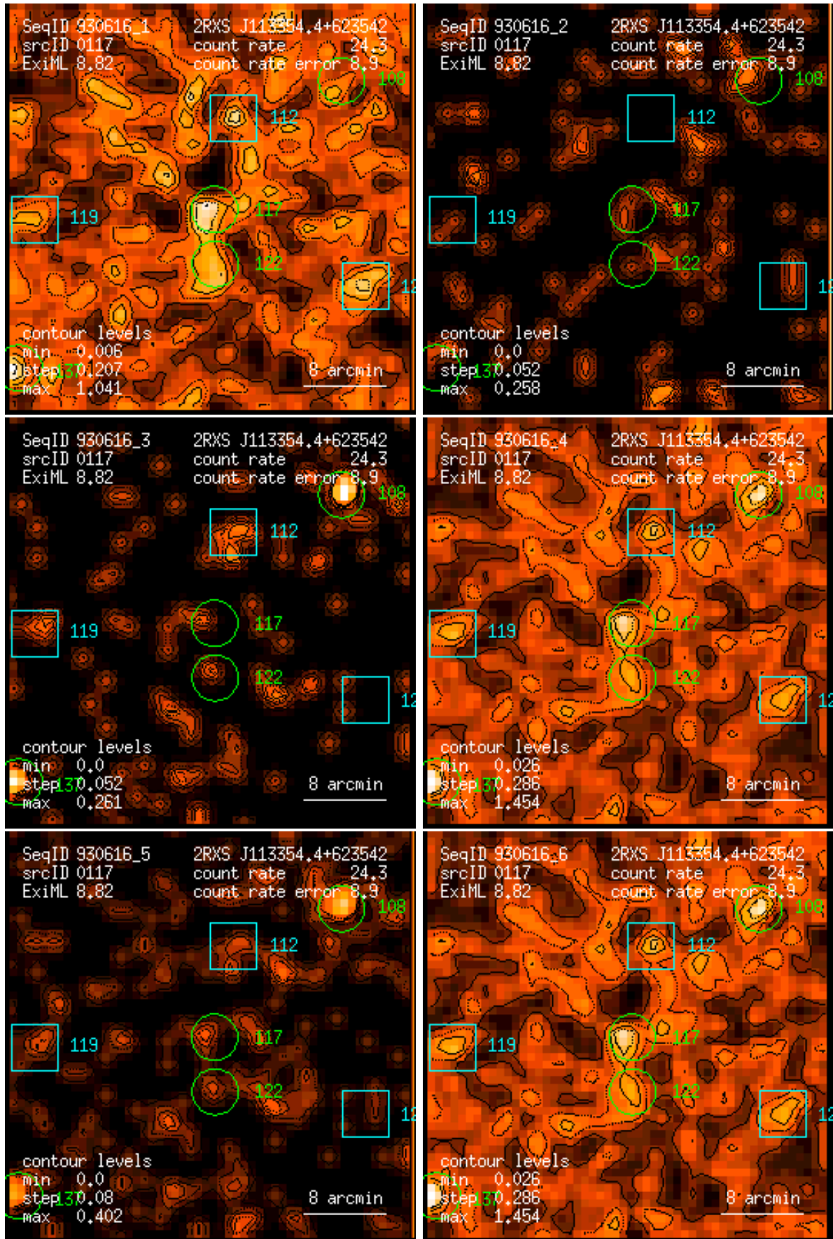
Figure 117: RASS 930616: detection 0117: band rate images, Gaussian filter: (1) PSPC channels 11 – 41, (2) 52 – 90, (3) 91 – 201, (4) 11 – 235, (5) 52 – 201, (6) 11 – 201. Broad band rates in counts/ks. Band rate contour levels in counts/ks/arcmin 2 .
