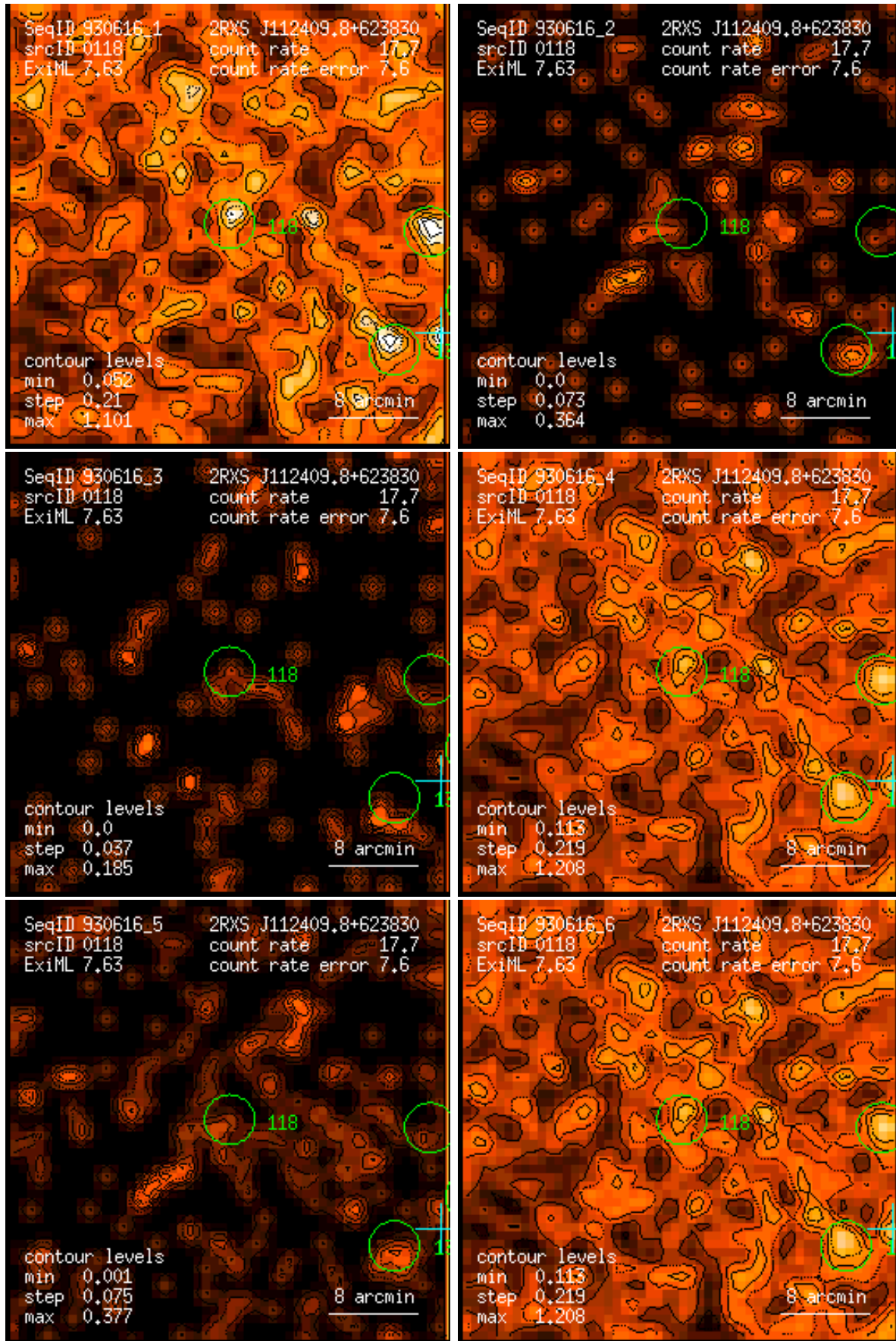
Figure 118: RASS 930616: detection 0118: band rate images, Gaussian filter: (1) PSPC channels 11 – 41, (2) 52 – 90, (3) 91 – 201, (4) 11 – 235, (5) 52 – 201, (6) 11 – 201. Broad band rates in counts/ks. Band rate contour levels in counts/ks/arcmin 2 .
