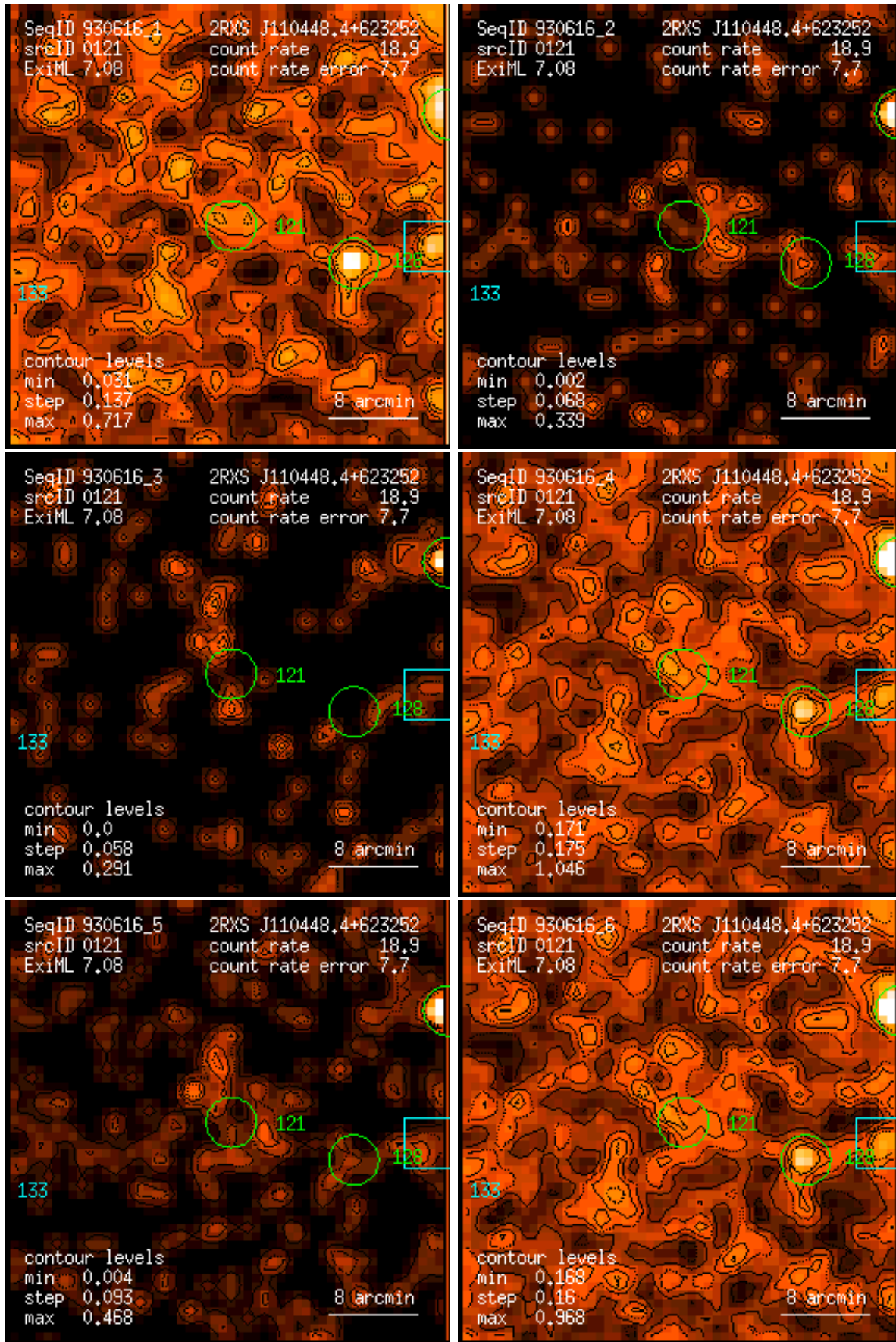
Figure 121: RASS 930616: detection 0121: band rate images, Gaussian filter: (1) PSPC channels 11 – 41, (2) 52 – 90, (3) 91 – 201, (4) 11 – 235, (5) 52 – 201, (6) 11 – 201. Broad band rates in counts/ks. Band rate contour levels in counts/ks/arcmin 2 .
