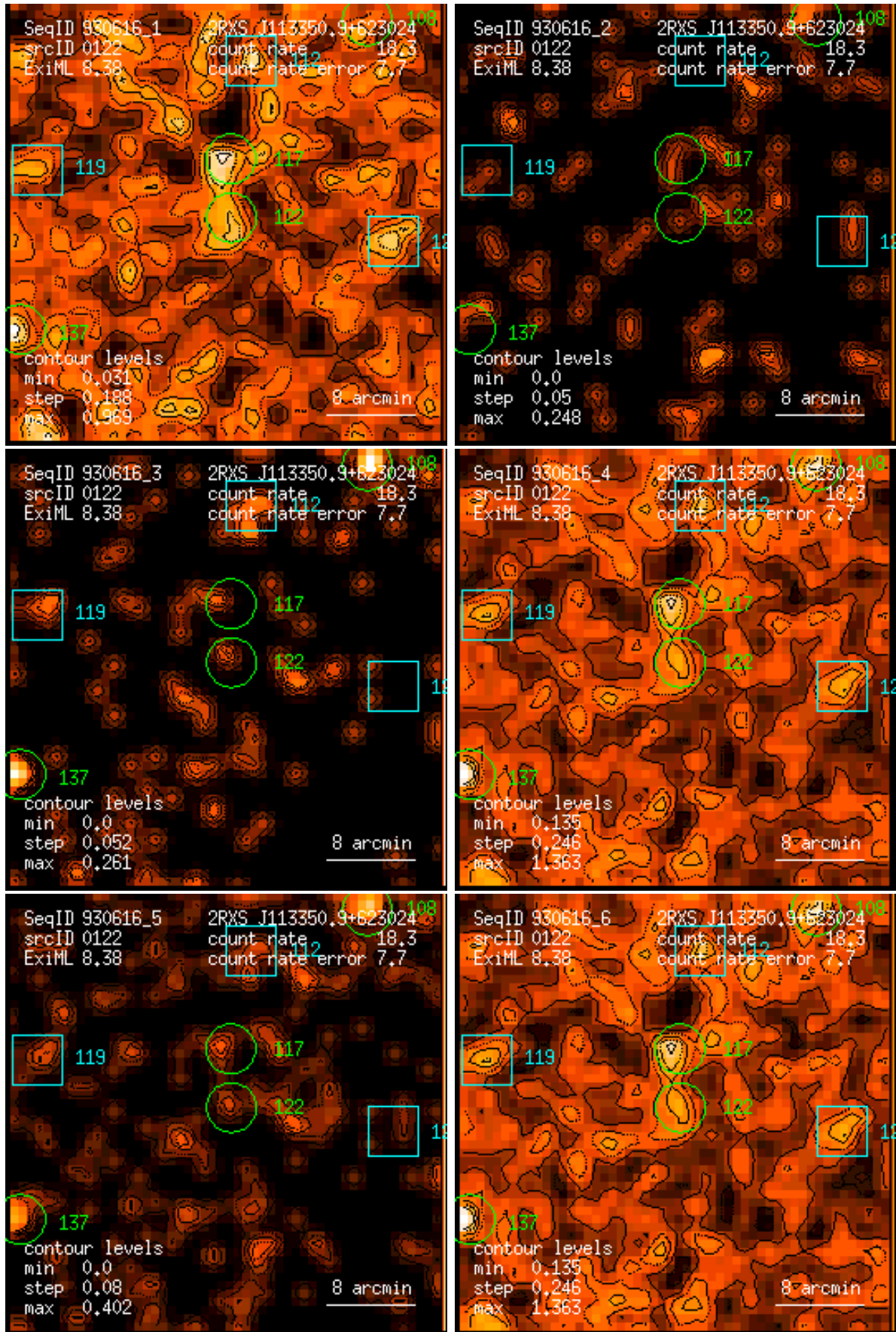
Figure 122: RASS 930616: detection 0122: band rate images, Gaussian filter: (1) PSPC channels 11 – 41, (2) 52 – 90, (3) 91 – 201, (4) 11 – 235, (5) 52 – 201, (6) 11 – 201. Broad band rates in counts/ks. Band rate contour levels in counts/ks/arcmin 2 .
