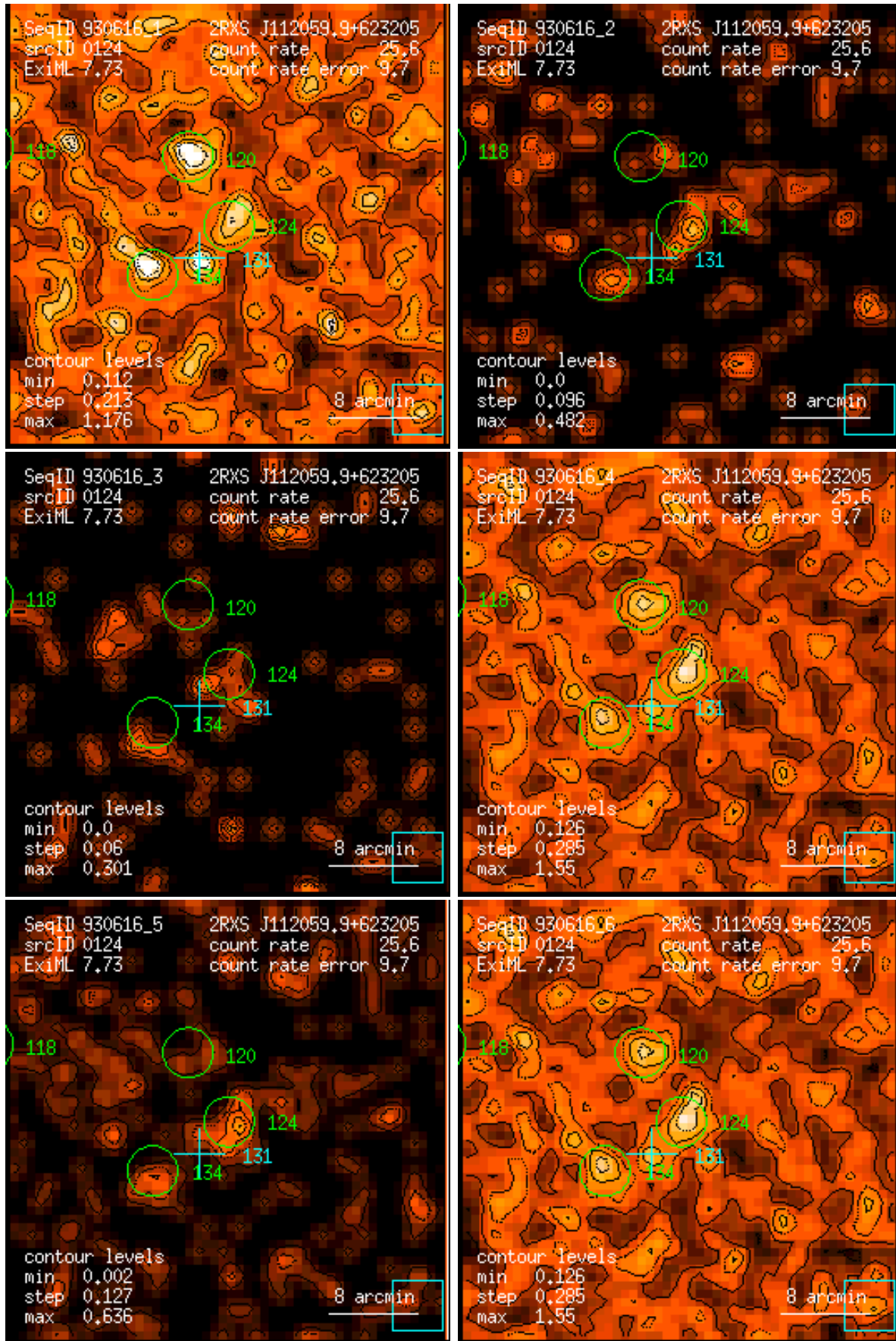
Figure 124: RASS 930616: detection 0124: band rate images, Gaussian filter: (1) PSPC channels 11 – 41, (2) 52 – 90, (3) 91 – 201, (4) 11 – 235, (5) 52 – 201, (6) 11 – 201. Broad band rates in counts/ks. Band rate contour levels in counts/ks/arcmin 2 .
