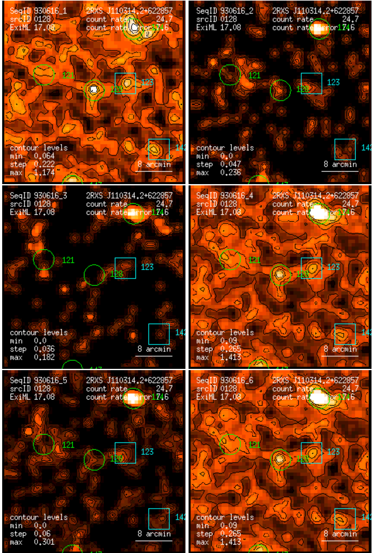
Figure 128: RASS 930616: detection 0128: band rate images, Gaussian filter: (1) PSPC channels 11 – 41, (2) 52 – 90, (3) 91 – 201, (4) 11 – 235, (5) 52 – 201, (6) 11 – 201. Broad band rates in counts/ks. Band rate contour levels in counts/ks/arcmin 2 .
