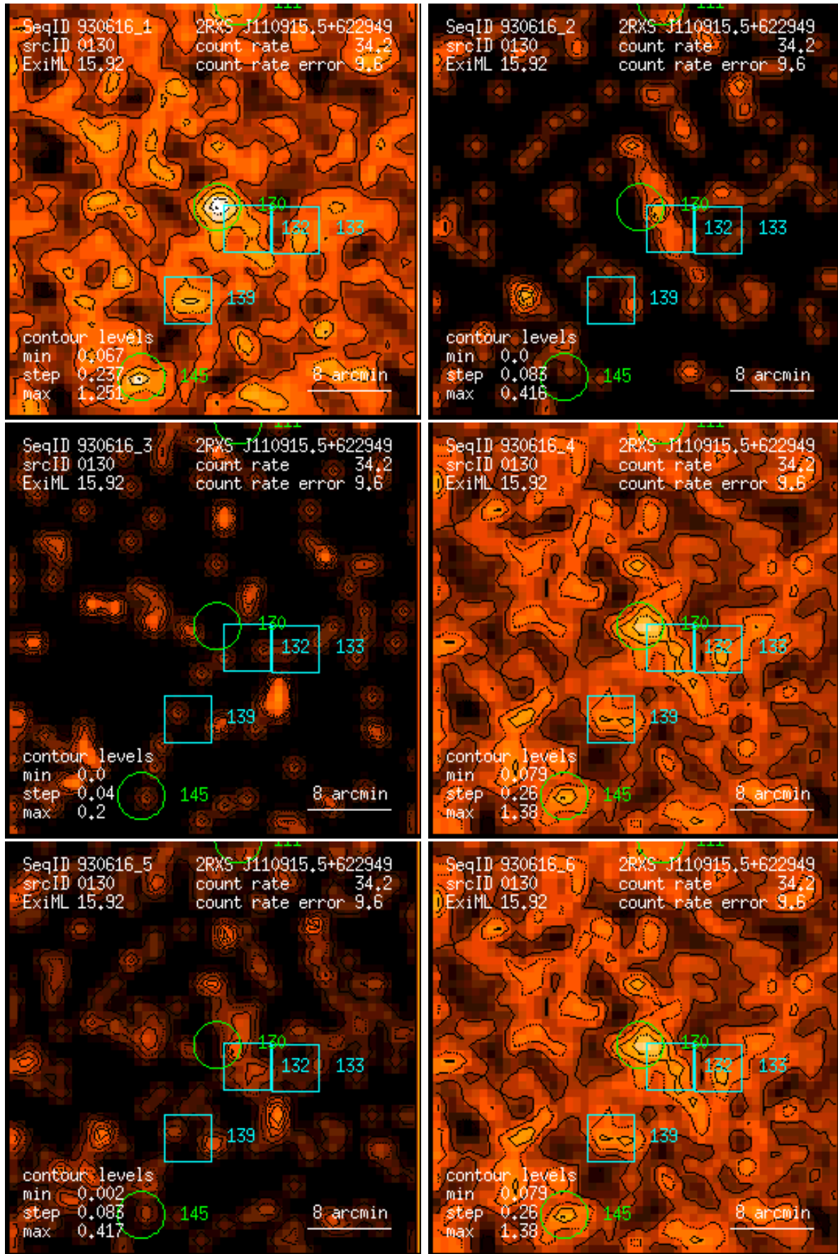
Figure 130: RASS 930616: detection 0130: band rate images, Gaussian filter: (1) PSPC channels 11 – 41, (2) 52 – 90, (3) 91 – 201, (4) 11 – 235, (5) 52 – 201, (6) 11 – 201. Broad band rates in counts/ks. Band rate contour levels in counts/ks/arcmin 2 .
