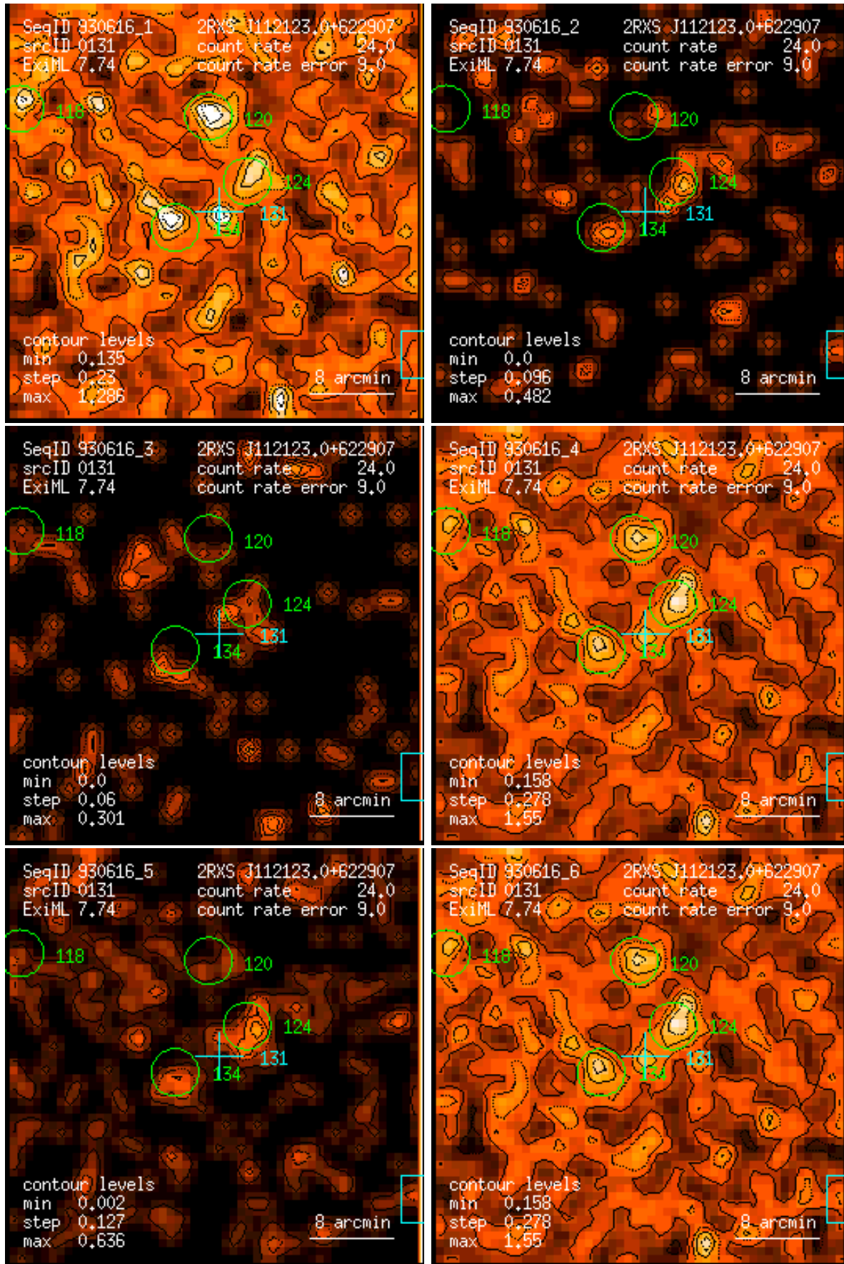
Figure 131: RASS 930616: detection 0131: band rate images, Gaussian filter: (1) PSPC channels 11 – 41, (2) 52 – 90, (3) 91 – 201, (4) 11 – 235, (5) 52 – 201, (6) 11 – 201. Broad band rates in counts/ks. Band rate contour levels in counts/ks/arcmin 2 .
