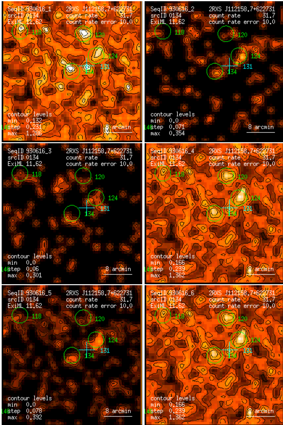
Figure 134: RASS 930616: detection 0134: band rate images, Gaussian filter: (1) PSPC channels 11 – 41, (2) 52 – 90, (3) 91 – 201, (4) 11 – 235, (5) 52 – 201, (6) 11 – 201. Broad band rates in counts/ks. Band rate contour levels in counts/ks/arcmin 2 .
