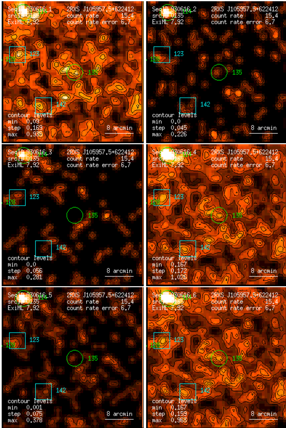
Figure 135: RASS 930616: detection 0135: band rate images, Gaussian filter: (1) PSPC channels 11 – 41, (2) 52 – 90, (3) 91 – 201, (4) 11 – 235, (5) 52 – 201, (6) 11 – 201. Broad band rates in counts/ks. Band rate contour levels in counts/ks/arcmin 2 .
