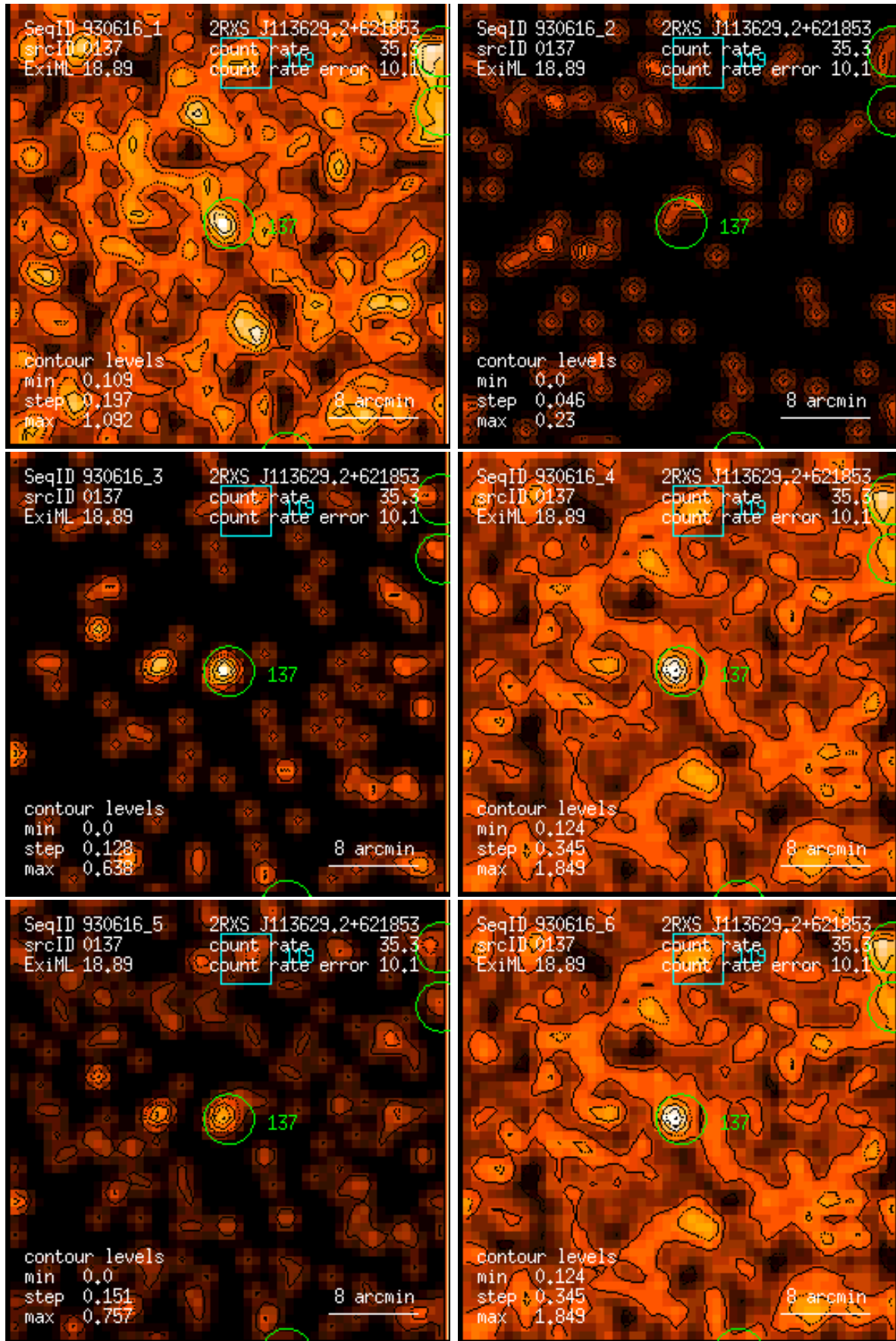
Figure 137: RASS 930616: detection 0137: band rate images, Gaussian filter: (1) PSPC channels 11 – 41, (2) 52 – 90, (3) 91 – 201, (4) 11 – 235, (5) 52 – 201, (6) 11 – 201. Broad band rates in counts/ks. Band rate contour levels in counts/ks/arcmin 2 .
