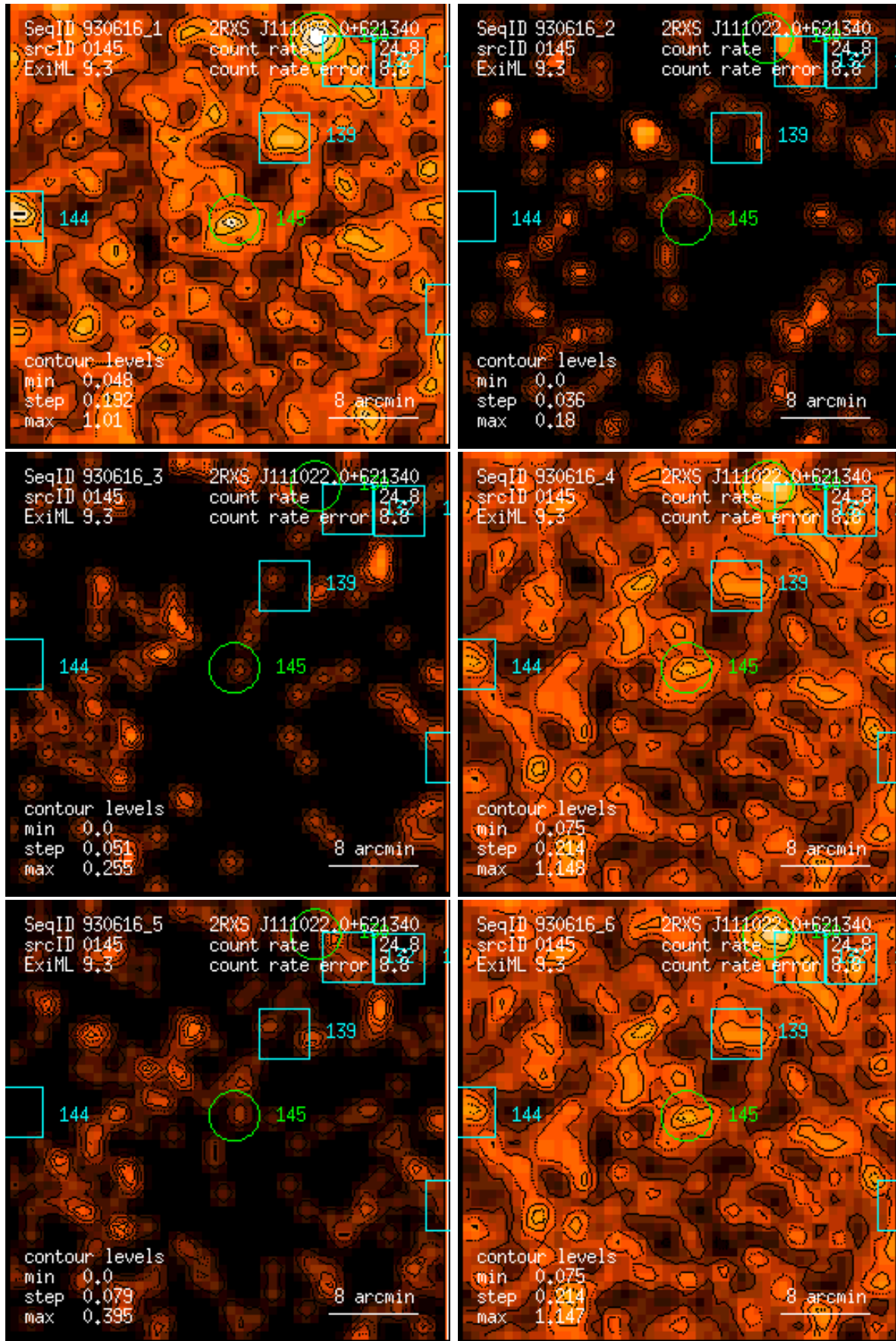
Figure 145: RASS 930616: detection 0145: band rate images, Gaussian filter: (1) PSPC channels 11 – 41, (2) 52 – 90, (3) 91 – 201, (4) 11 – 235, (5) 52 – 201, (6) 11 – 201. Broad band rates in counts/ks. Band rate contour levels in counts/ks/arcmin 2 .
