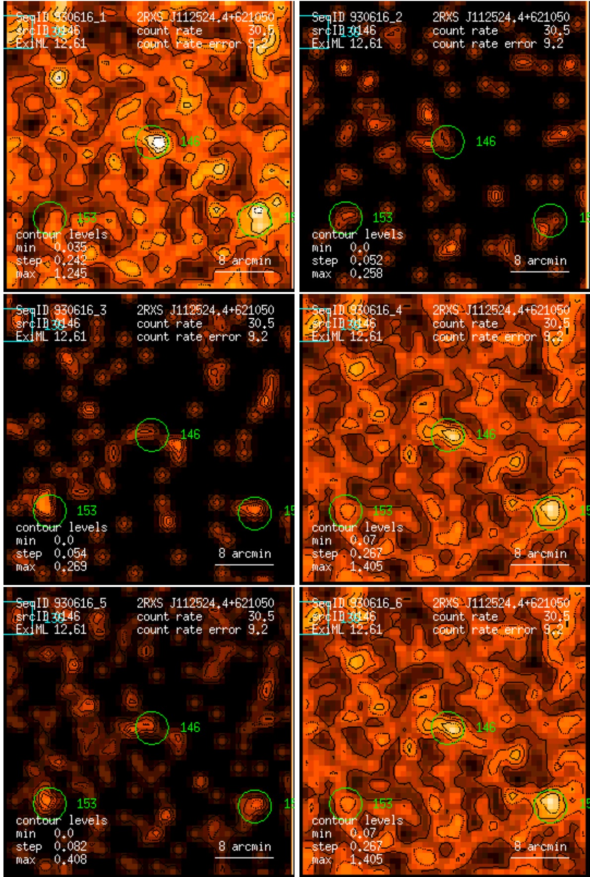
Figure 146: RASS 930616: detection 0146: band rate images, Gaussian filter: (1) PSPC channels 11 – 41, (2) 52 – 90, (3) 91 – 201, (4) 11 – 235, (5) 52 – 201, (6) 11 – 201. Broad band rates in counts/ks. Band rate contour levels in counts/ks/arcmin 2 .
