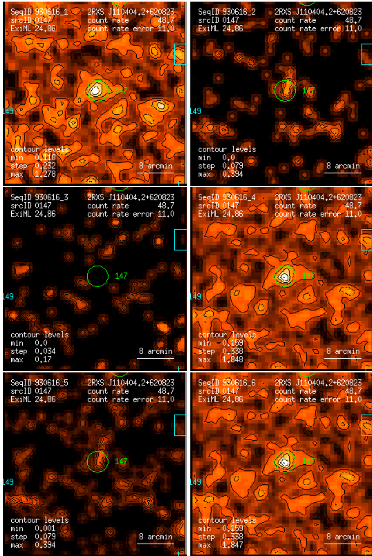
Figure 147: RASS 930616: detection 0147: band rate images, Gaussian filter: (1) PSPC channels 11 – 41, (2) 52 – 90, (3) 91 – 201, (4) 11 – 235, (5) 52 – 201, (6) 11 – 201. Broad band rates in counts/ks. Band rate contour levels in counts/ks/arcmin 2 .
