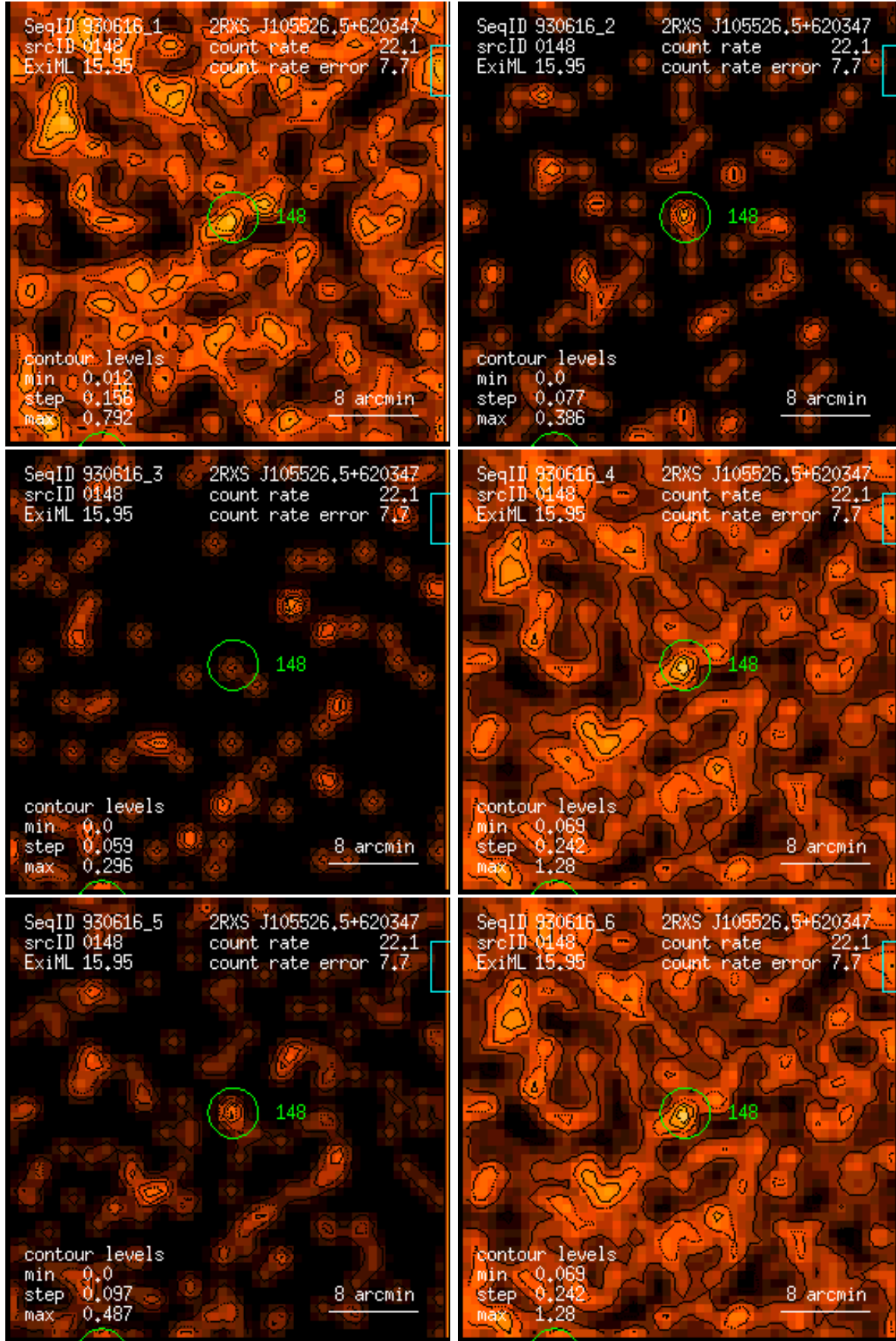
Figure 148: RASS 930616: detection 0148: band rate images, Gaussian filter: (1) PSPC channels 11 – 41, (2) 52 – 90, (3) 91 – 201, (4) 11 – 235, (5) 52 – 201, (6) 11 – 201. Broad band rates in counts/ks. Band rate contour levels in counts/ks/arcmin 2 .
