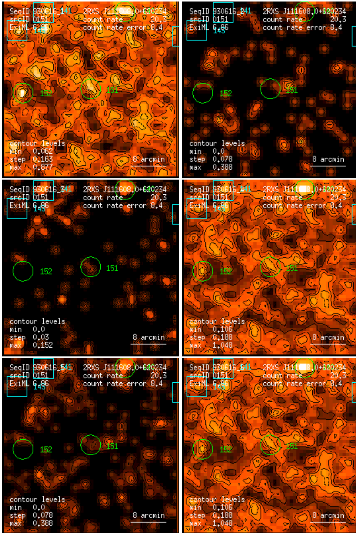
Figure 151: RASS 930616: detection 0151: band rate images, Gaussian filter: (1) PSPC channels 11 – 41, (2) 52 – 90, (3) 91 – 201, (4) 11 – 235, (5) 52 – 201, (6) 11 – 201. Broad band rates in counts/ks. Band rate contour levels in counts/ks/arcmin 2 .
