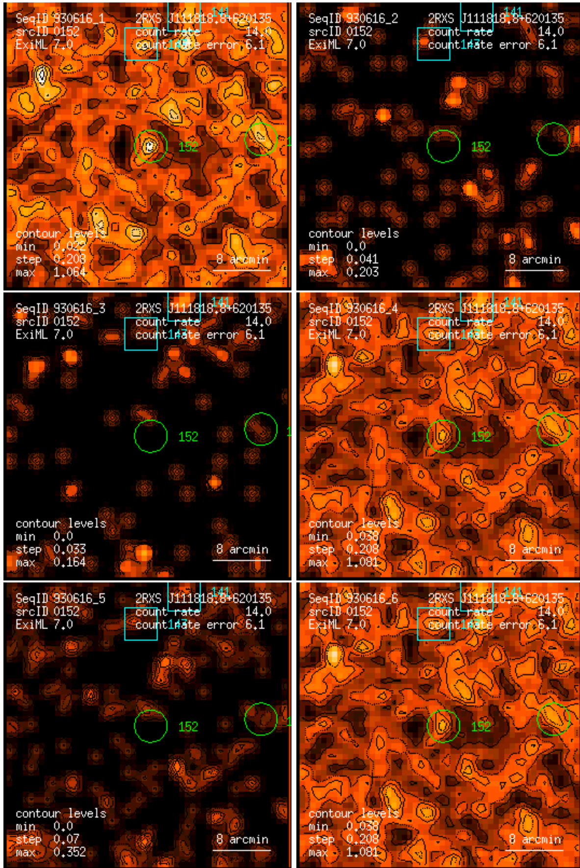
Figure 152: RASS 930616: detection 0152: band rate images, Gaussian filter: (1) PSPC channels 11 – 41, (2) 52 – 90, (3) 91 – 201, (4) 11 – 235, (5) 52 – 201, (6) 11 – 201. Broad band rates in counts/ks. Band rate contour levels in counts/ks/arcmin 2 .
