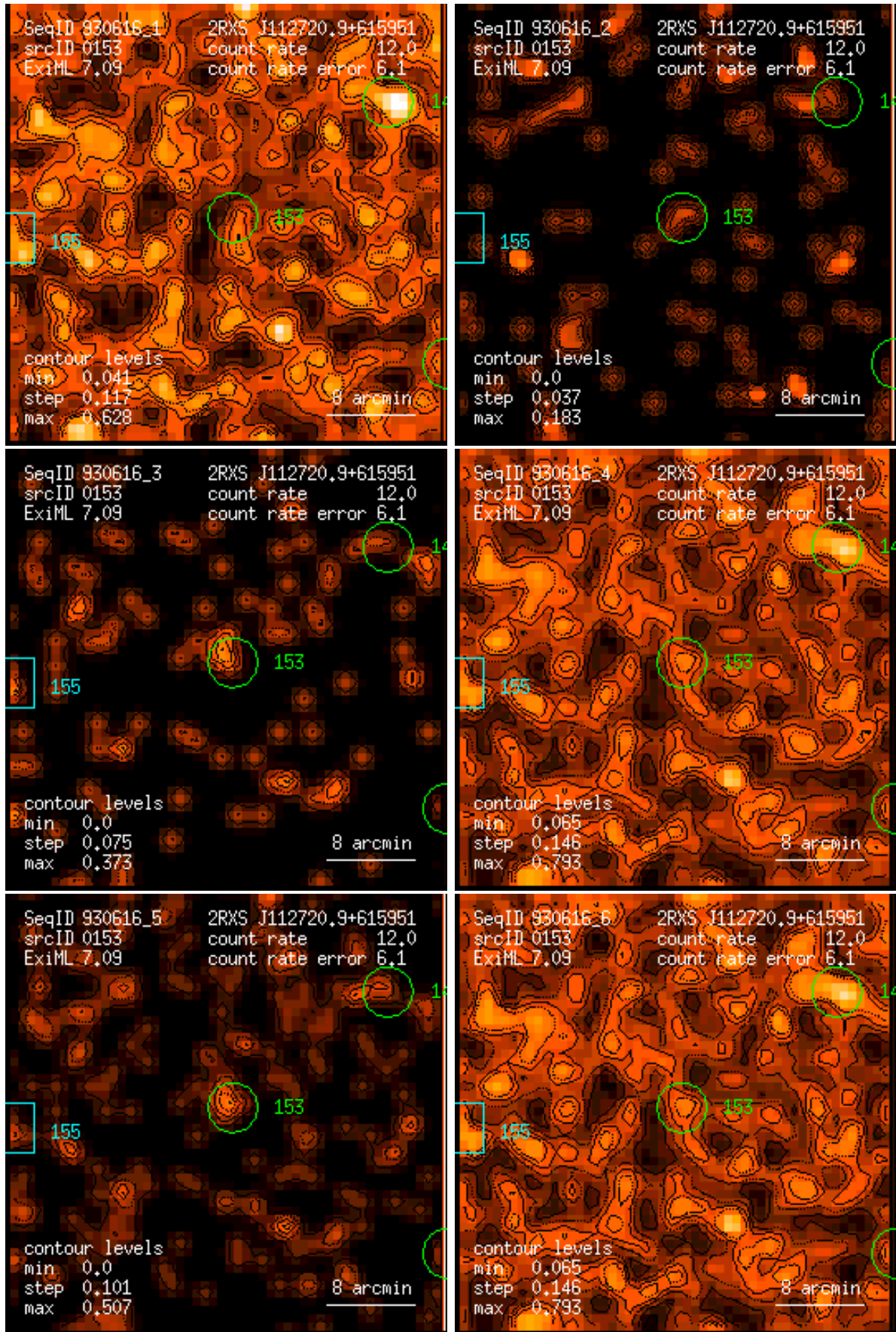
Figure 153: RASS 930616: detection 0153: band rate images, Gaussian filter: (1) PSPC channels 11 – 41, (2) 52 – 90, (3) 91 – 201, (4) 11 – 235, (5) 52 – 201, (6) 11 – 201. Broad band rates in counts/ks. Band rate contour levels in counts/ks/arcmin 2 .
