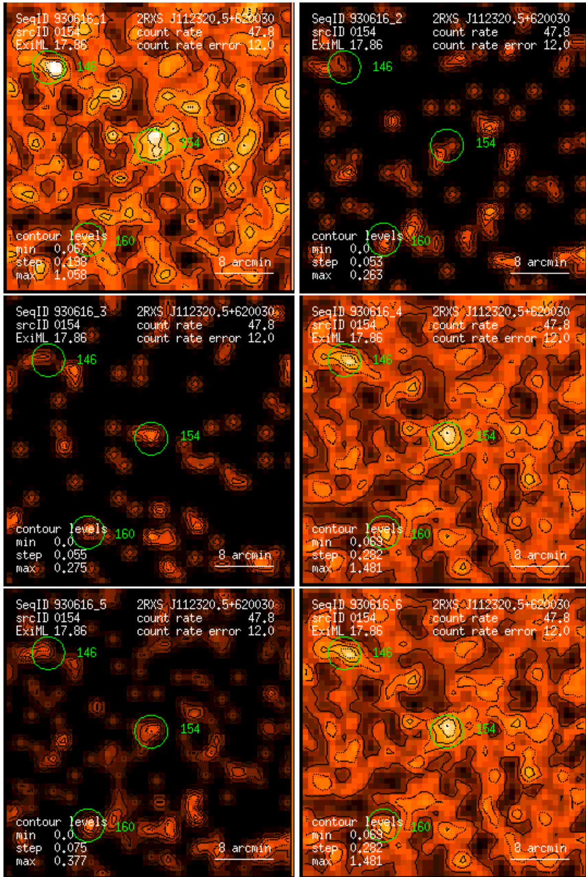
Figure 154: RASS 930616: detection 0154: band rate images, Gaussian filter: (1) PSPC channels 11 – 41, (2) 52 – 90, (3) 91 – 201, (4) 11 – 235, (5) 52 – 201, (6) 11 – 201. Broad band rates in counts/ks. Band rate contour levels in counts/ks/arcmin 2 .
