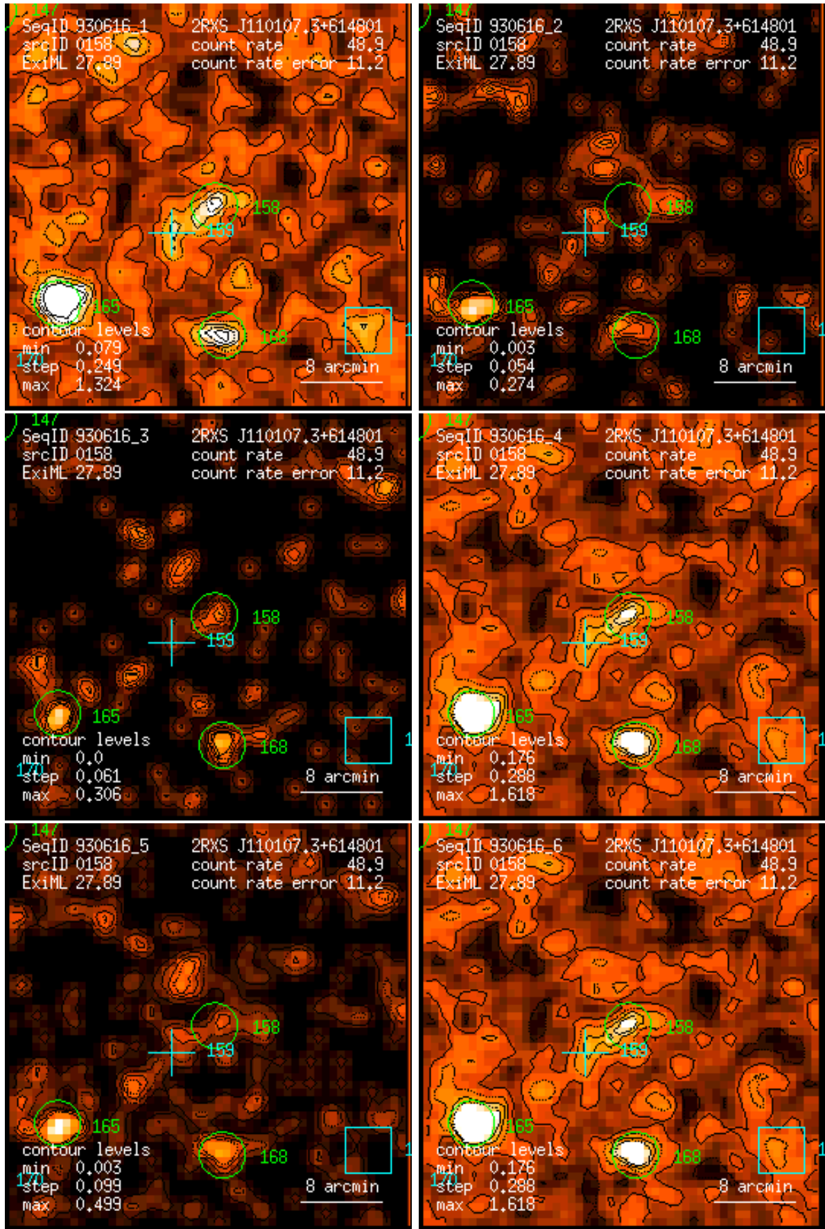
Figure 158: RASS 930616: detection 0158: band rate images, Gaussian filter: (1) PSPC channels 11 – 41, (2) 52 – 90, (3) 91 – 201, (4) 11 – 235, (5) 52 – 201, (6) 11 – 201. Broad band rates in counts/ks. Band rate contour levels in counts/ks/arcmin 2 .
