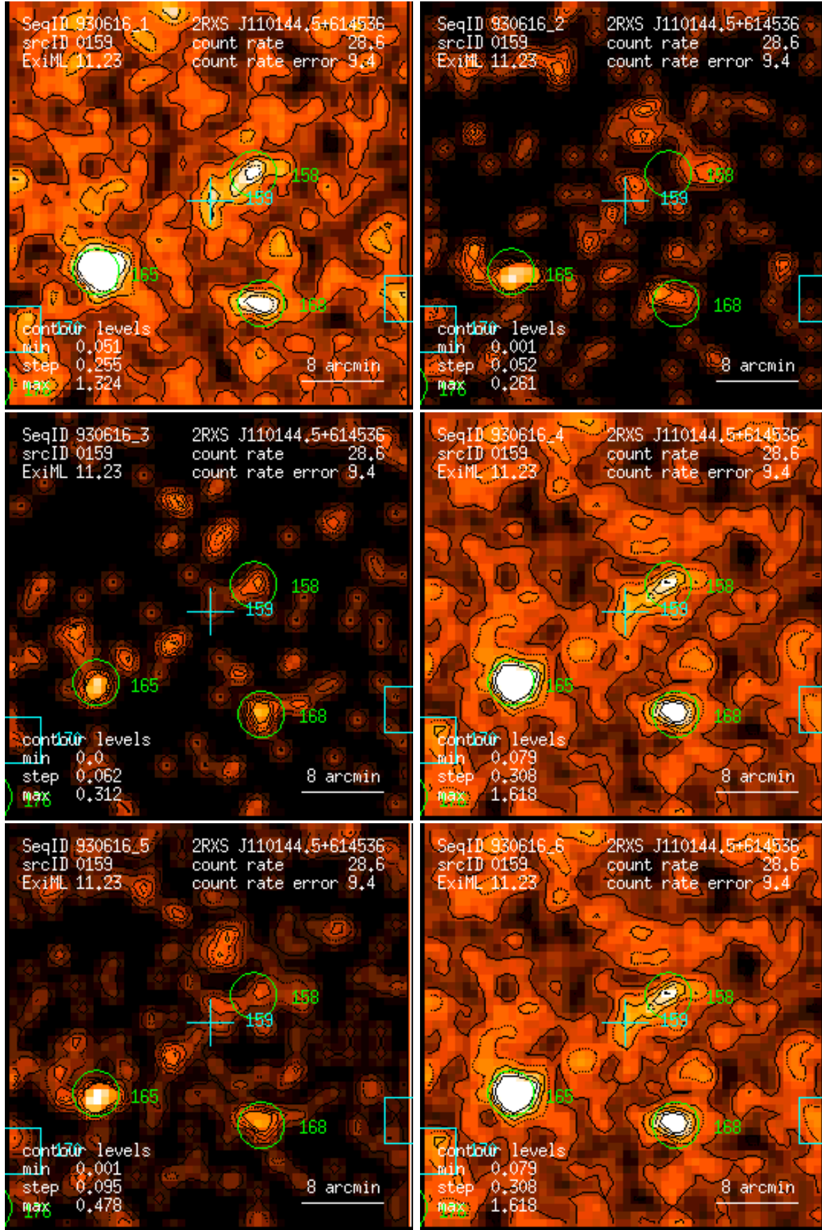
Figure 159: RASS 930616: detection 0159: band rate images, Gaussian filter: (1) PSPC channels 11 – 41, (2) 52 – 90, (3) 91 – 201, (4) 11 – 235, (5) 52 – 201, (6) 11 – 201. Broad band rates in counts/ks. Band rate contour levels in counts/ks/arcmin 2 .
