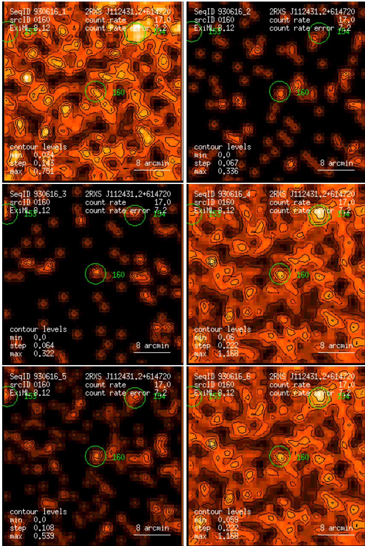
Figure 160: RASS 930616: detection 0160: band rate images, Gaussian filter: (1) PSPC channels 11 – 41, (2) 52 – 90, (3) 91 – 201, (4) 11 – 235, (5) 52 – 201, (6) 11 – 201. Broad band rates in counts/ks. Band rate contour levels in counts/ks/arcmin 2 .
