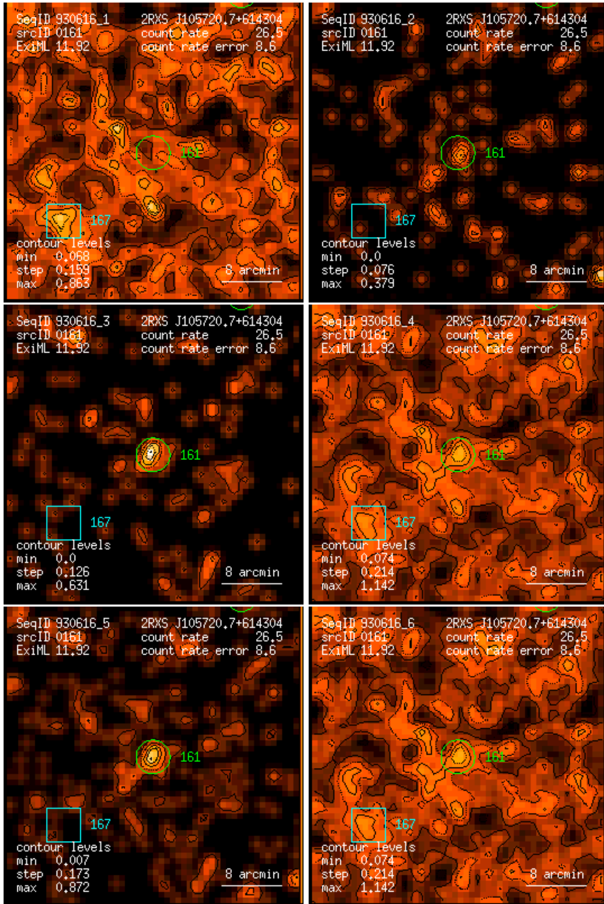
Figure 161: RASS 930616: detection 0161: band rate images, Gaussian filter: (1) PSPC channels 11 – 41, (2) 52 – 90, (3) 91 – 201, (4) 11 – 235, (5) 52 – 201, (6) 11 – 201. Broad band rates in counts/ks. Band rate contour levels in counts/ks/arcmin 2 .
