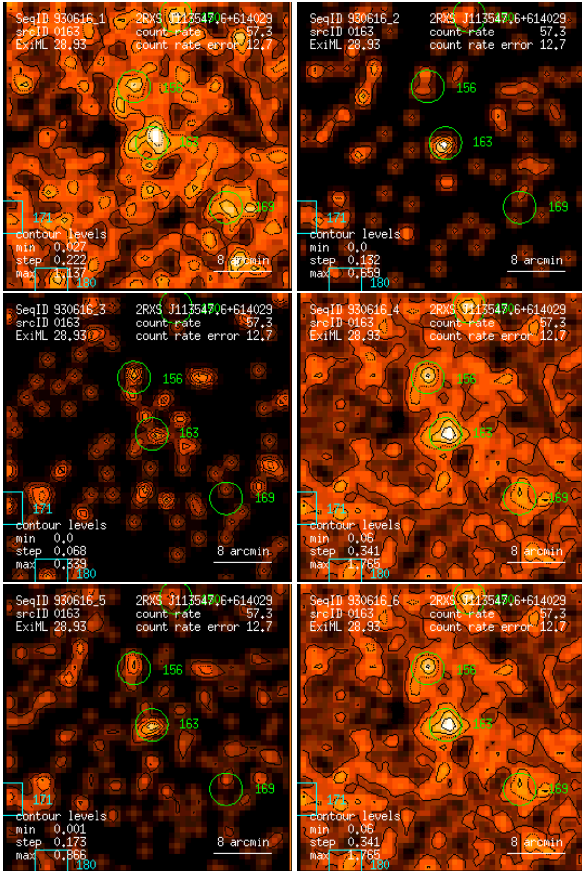
Figure 163: RASS 930616: detection 0163: band rate images, Gaussian filter: (1) PSPC channels 11 – 41, (2) 52 – 90, (3) 91 – 201, (4) 11 – 235, (5) 52 – 201, (6) 11 – 201. Broad band rates in counts/ks. Band rate contour levels in counts/ks/arcmin 2 .
