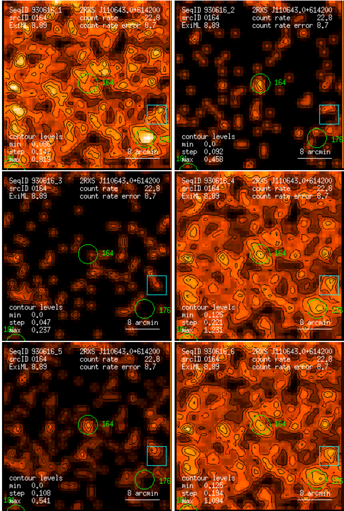
Figure 164: RASS 930616: detection 0164: band rate images, Gaussian filter: (1) PSPC channels 11 – 41, (2) 52 – 90, (3) 91 – 201, (4) 11 – 235, (5) 52 – 201, (6) 11 – 201. Broad band rates in counts/ks. Band rate contour levels in counts/ks/arcmin 2 .
