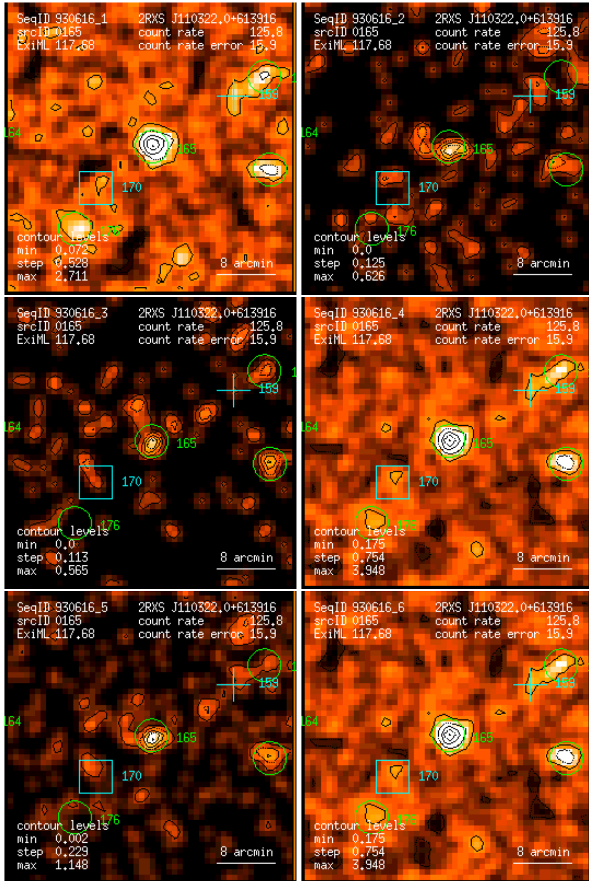
Figure 165: RASS 930616: detection 0165: band rate images, Gaussian filter: (1) PSPC channels 11 – 41, (2) 52 – 90, (3) 91 – 201, (4) 11 – 235, (5) 52 – 201, (6) 11 – 201. Broad band rates in counts/ks. Band rate contour levels in counts/ks/arcmin 2 .
