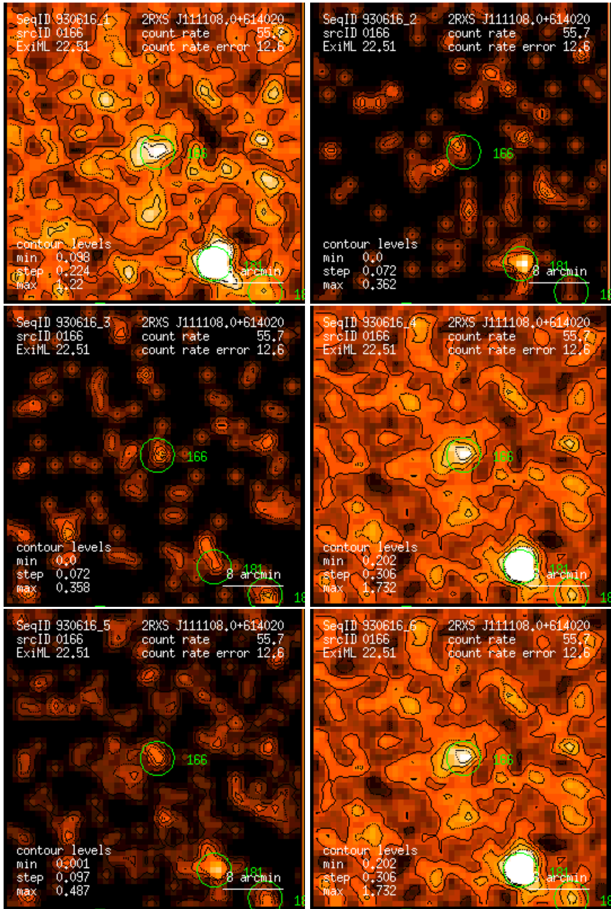
Figure 166: RASS 930616: detection 0166: band rate images, Gaussian filter: (1) PSPC channels 11 – 41, (2) 52 – 90, (3) 91 – 201, (4) 11 – 235, (5) 52 – 201, (6) 11 – 201. Broad band rates in counts/ks. Band rate contour levels in counts/ks/arcmin 2 .
