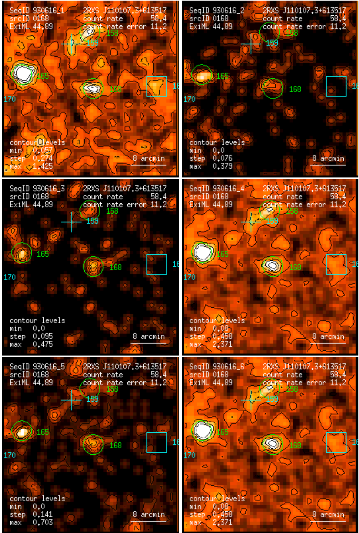
Figure 168: RASS 930616: detection 0168: band rate images, Gaussian filter: (1) PSPC channels 11 – 41, (2) 52 – 90, (3) 91 – 201, (4) 11 – 235, (5) 52 – 201, (6) 11 – 201. Broad band rates in counts/ks. Band rate contour levels in counts/ks/arcmin 2 .
