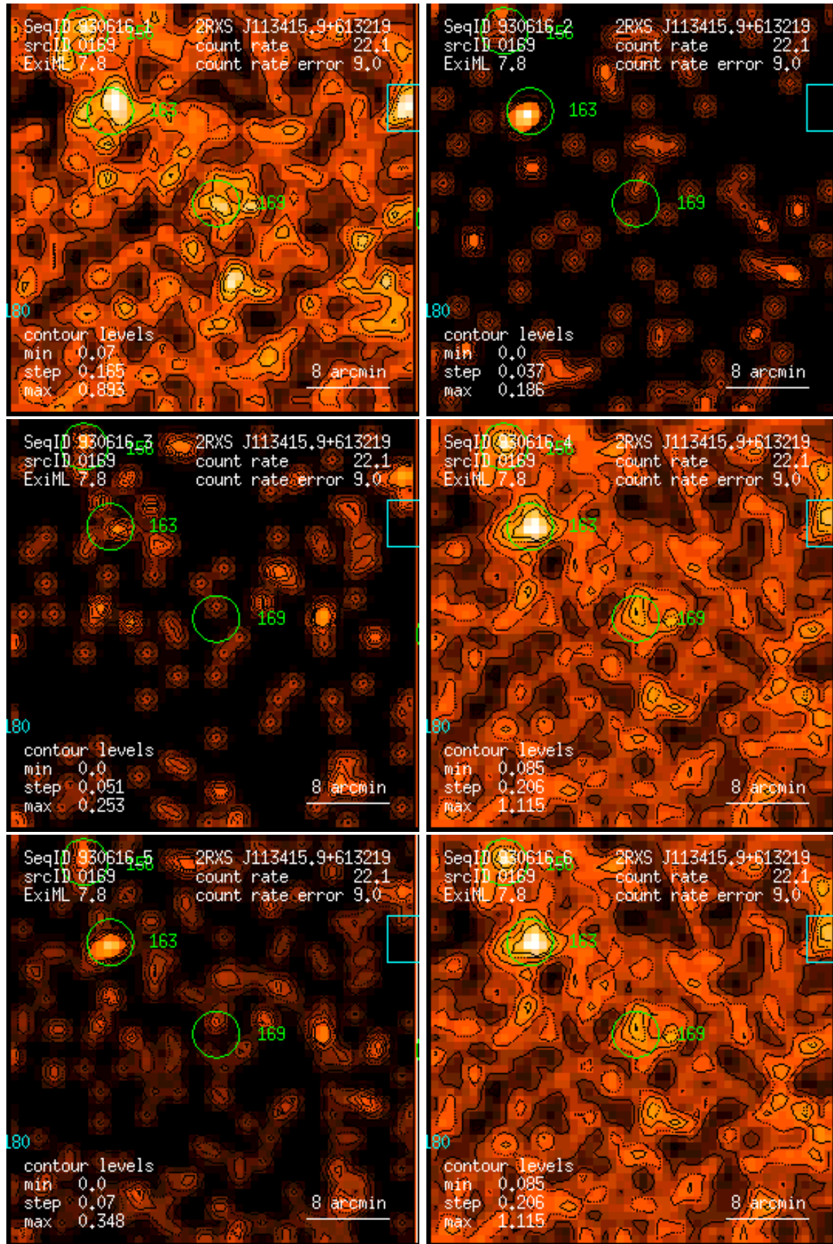
Figure 169: RASS 930616: detection 0169: band rate images, Gaussian filter: (1) PSPC channels 11 – 41, (2) 52 – 90, (3) 91 – 201, (4) 11 – 235, (5) 52 – 201, (6) 11 – 201. Broad band rates in counts/ks. Band rate contour levels in counts/ks/arcmin 2 .
