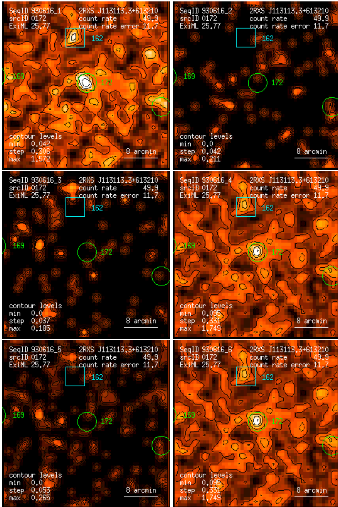
Figure 172: RASS 930616: detection 0172: band rate images, Gaussian filter: (1) PSPC channels 11 – 41, (2) 52 – 90, (3) 91 – 201, (4) 11 – 235, (5) 52 – 201, (6) 11 – 201. Broad band rates in counts/ks. Band rate contour levels in counts/ks/arcmin 2 .
